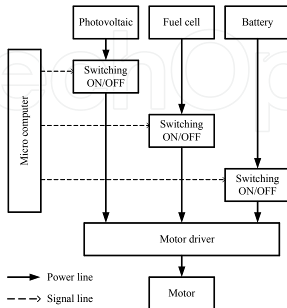
Fig. 7. Concept of energy control system
