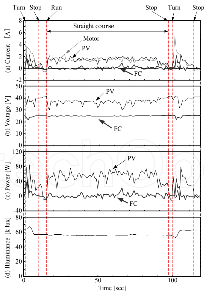
Fig. 11. Experimental results (Low Speed mode, Low)
