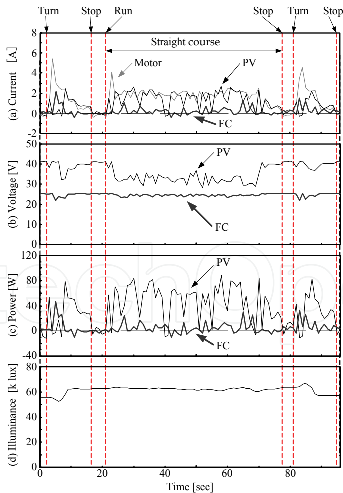
Fig. 12. Experimental results (Low Speed mode, High)
