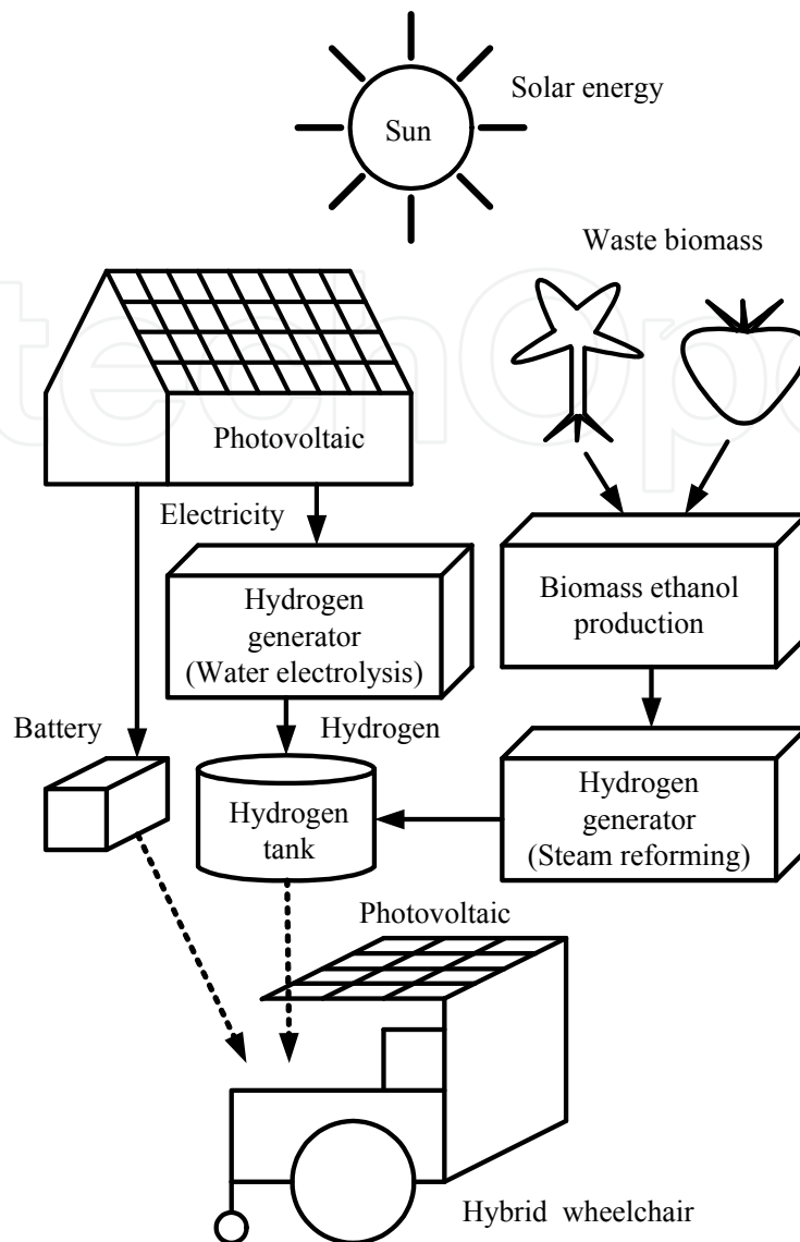
Fig. 2. Schematic explanation of energy flow
