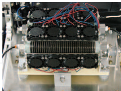
(a) Fuel cell and vibration isolator
