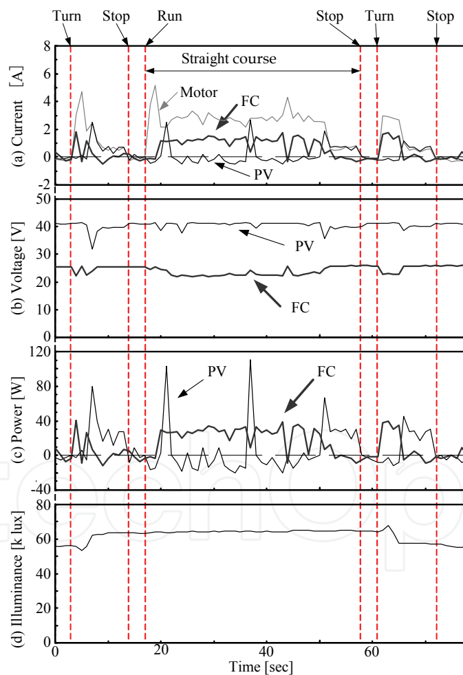
Fig. 14. Experimental results (High Speed mode, High)
