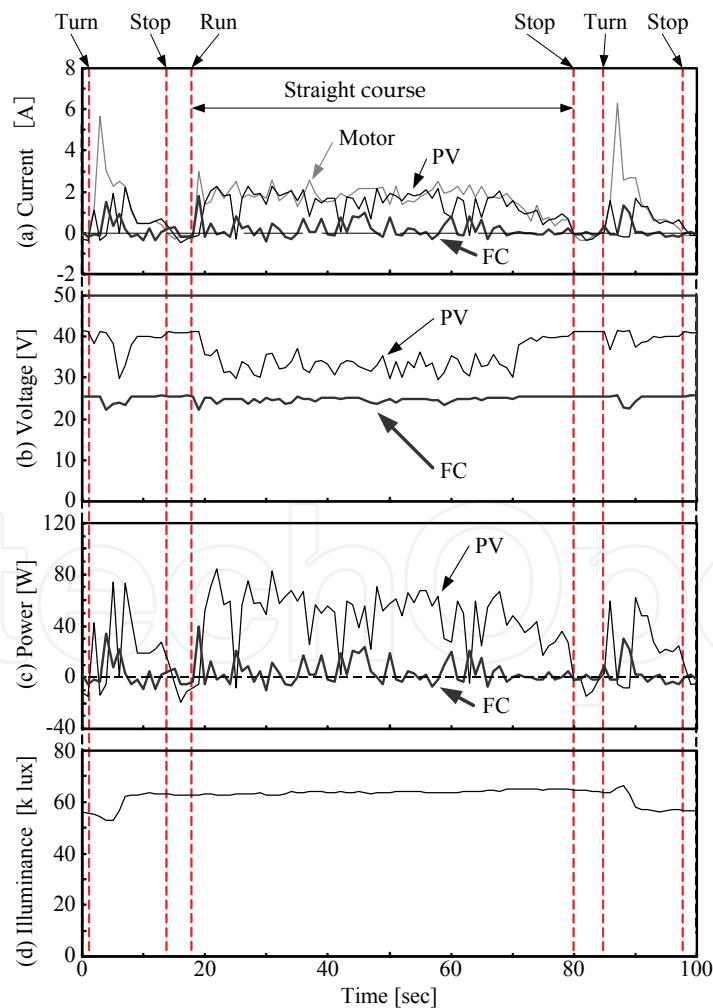
Fig. 13. Experimental results (High Speed mode, Low)
