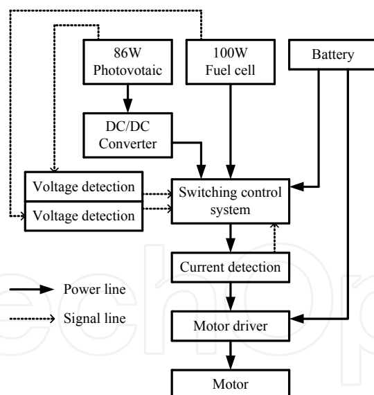
Fig. 8. Detailed energy control architecture
