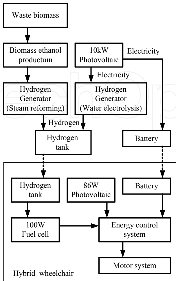
Fig. 3. Block diagram of energy flow
