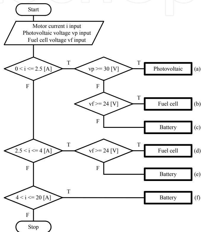
Fig. 9. Software control algorithm of energy control system
