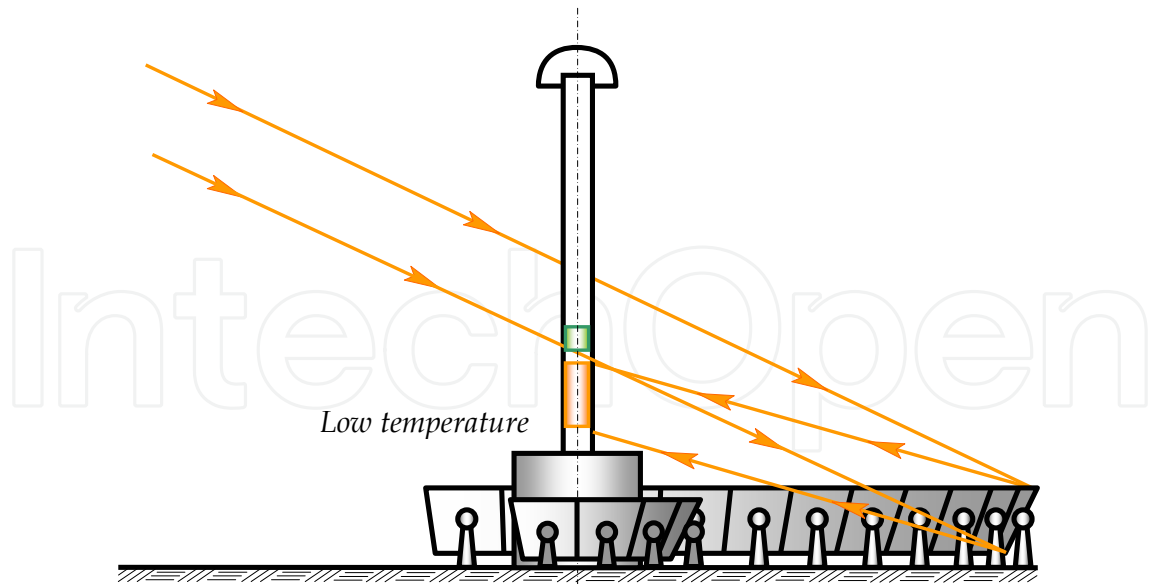
Fig. 7. Solar array concept for the closed-circuit thermal-gravity tower.
