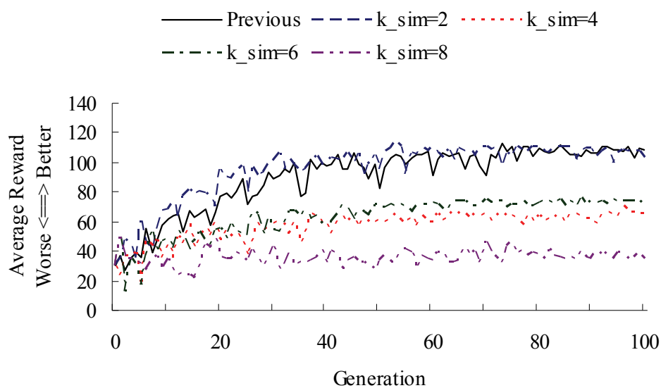
Fig. 6. Gain attained by Q-learning generated by QDSEGA
