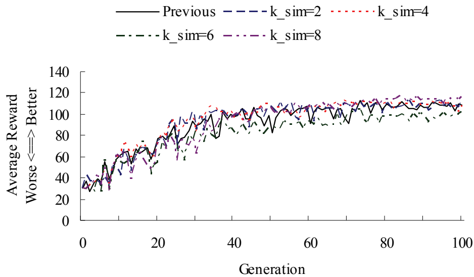
Fig. 8. Gain attained by Q-learning generated by QDSEGA applied the neighboring crossover when obtaining 100 reward
