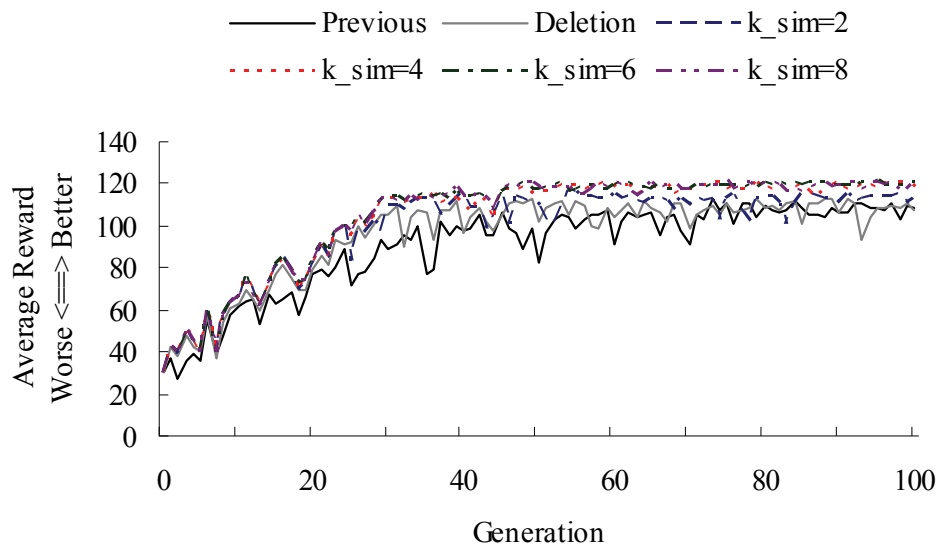
Fig. 10. Gain attained by Q-learning generated by QDSEGA applied the neighboring crossover and the deletion algorithm when obtaining 100 reward
