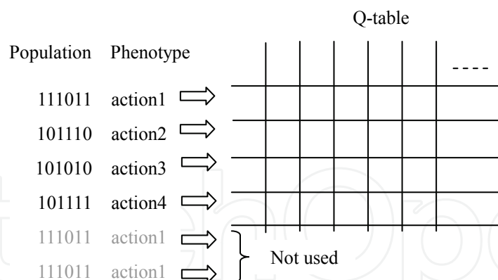
Fig. 2. Q-table created from a set of individuals
