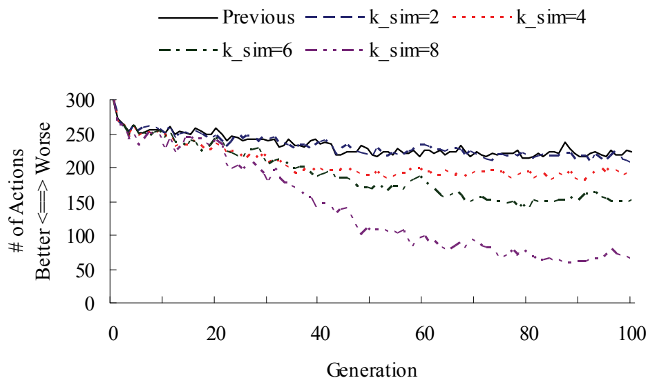
Fig. 9. The number of actions in Q-table generated by QDSEGA applied the neighboring crossover when obtaining 100 reward
