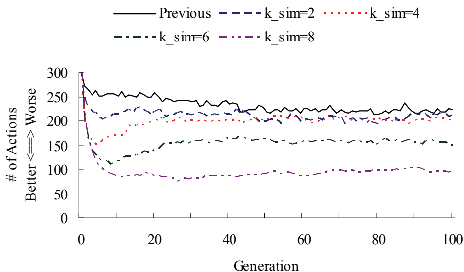
Fig. 7. The number of actions in Q-table generated by QDSEGA
