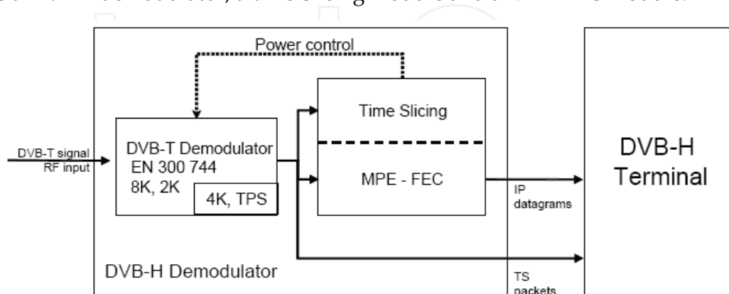
Fig. 1. Conceptual structure of a DVB-H receiver.
