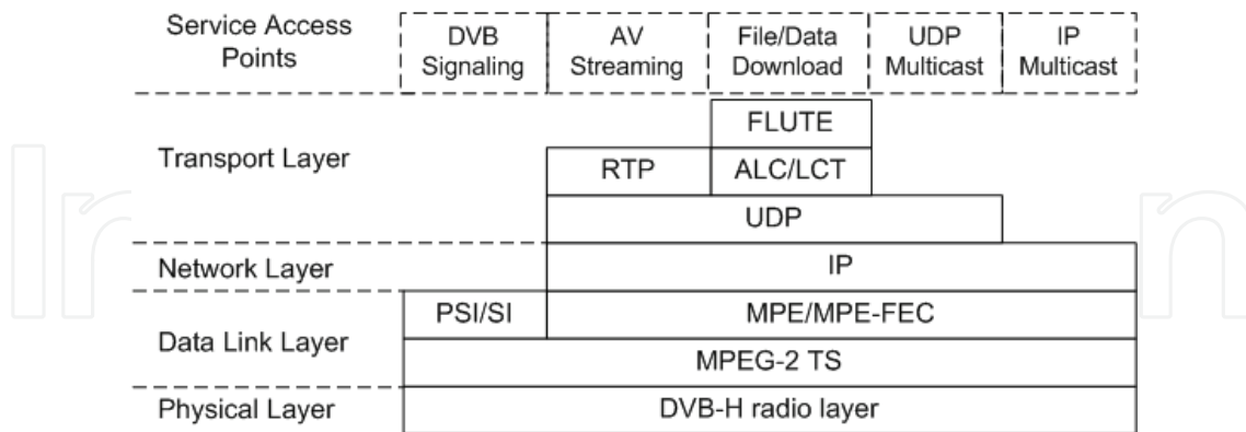
Fig. 3. The DVB-IPDC protocol stack.
