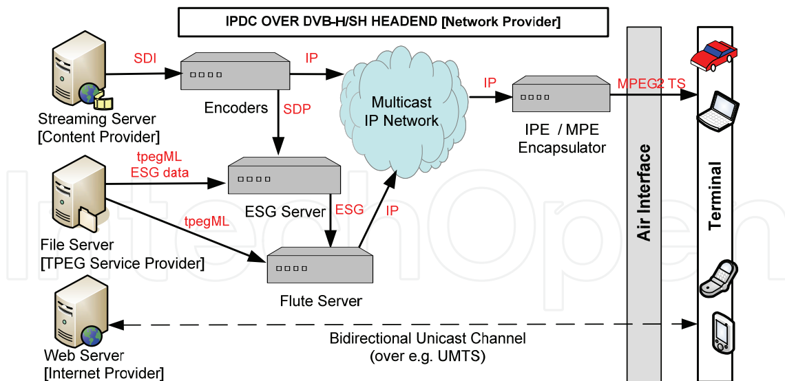
Fig. 8. Coupling of the TPEG Service Provider with the IPDC over DVB-H/SH headend
