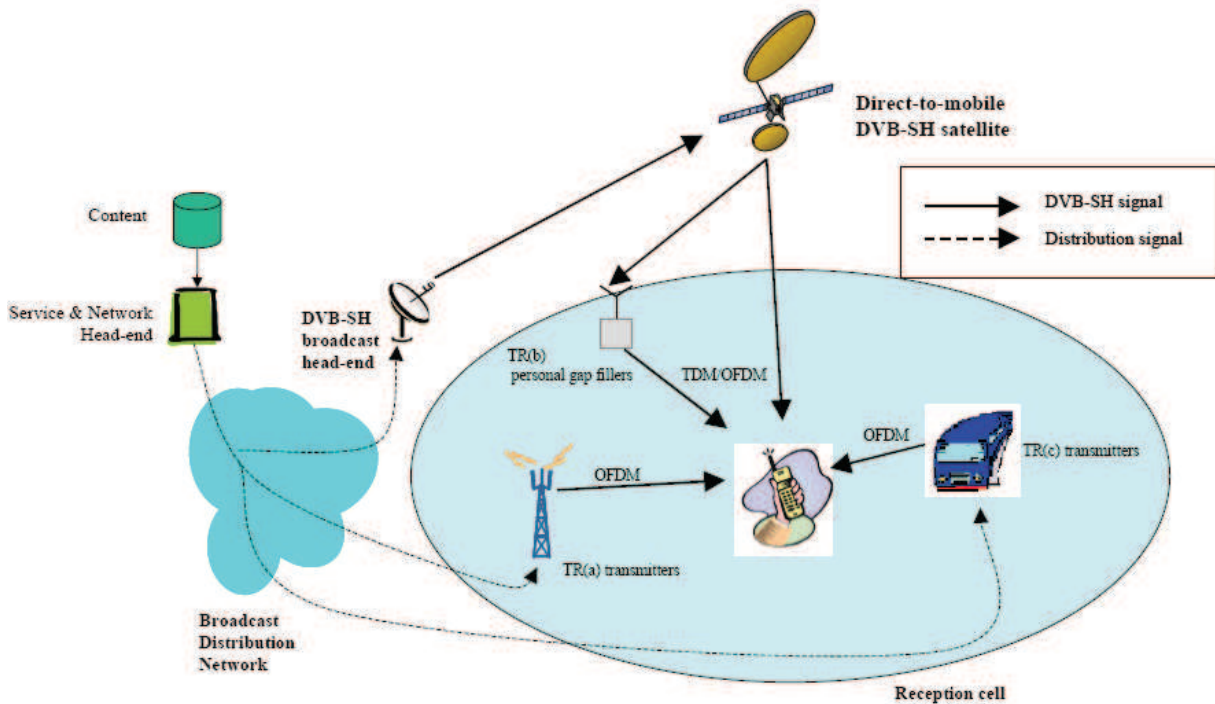
Fig. 2. Overall DVB-SH system architecture.
