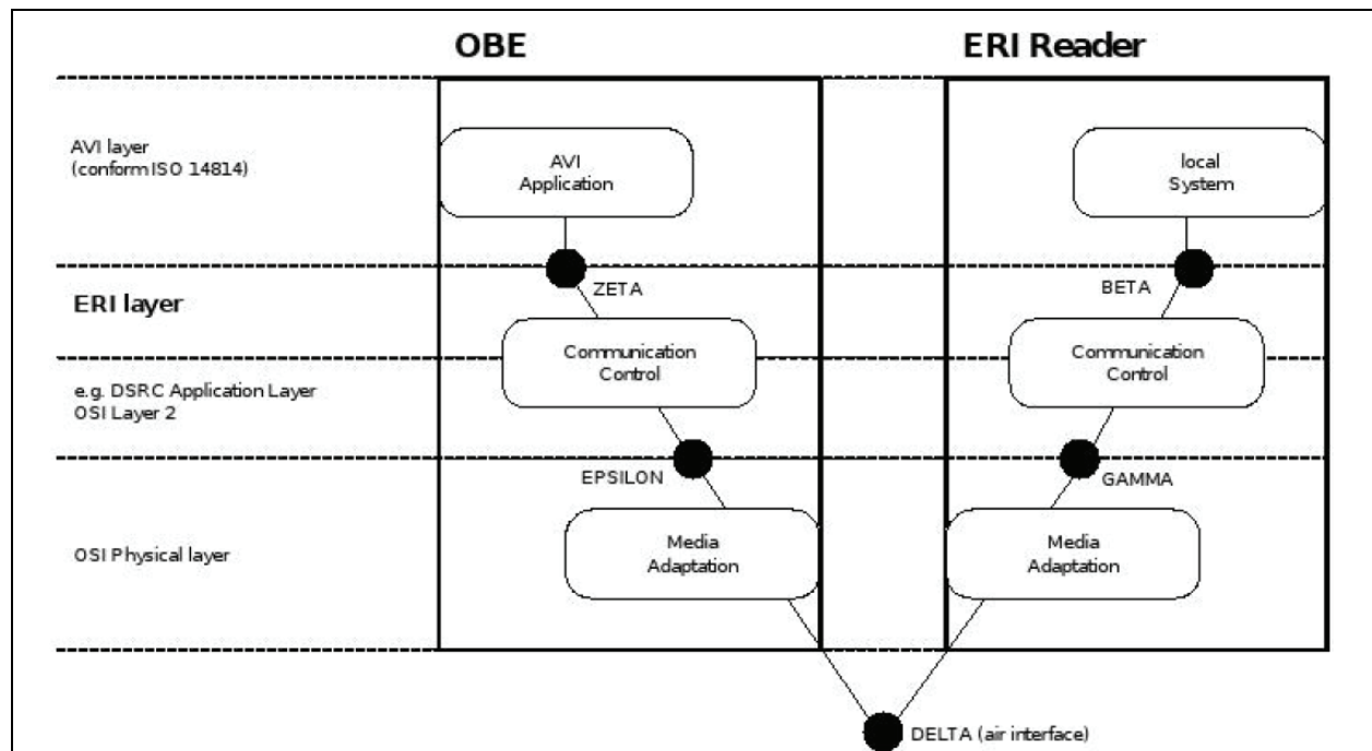
Fig. 1. ERI within the AVI/AEI reference architecture framework.
