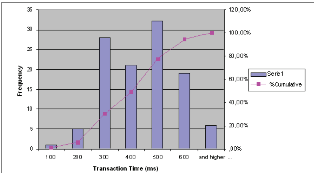
Fig. 11. Histogram with transaction times for WiFi technology.
