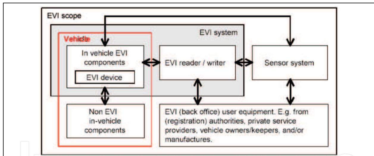
Fig. 2. Schema of components in the EVI scope
