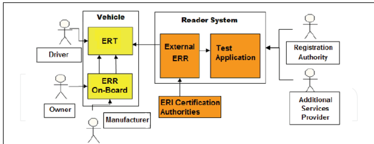
Fig. 6. Schema of the identification system.
