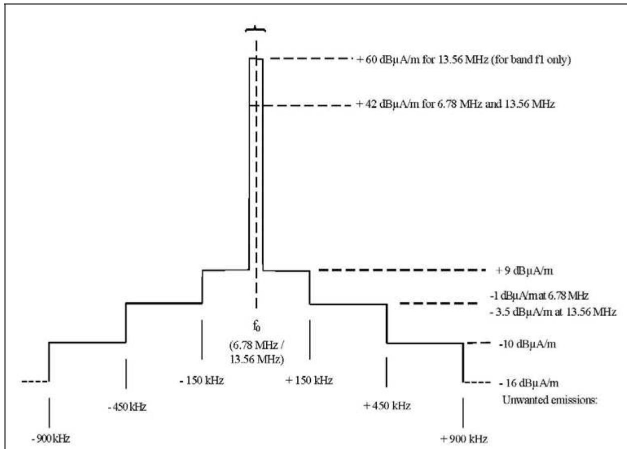
Fig. 9. ISM frequencies for 6.78MHz and 13.56MHz
