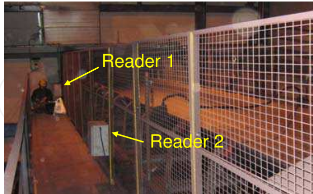
Fig. 5. The position of the two RFID readers used for the second set of tests. Reader ones antenna is mounted under the conveyor but bend slightly as a saddle so the distance between the conveyor and the antenna was minimized. Reader twos antenna is mounted around the conveyor.
