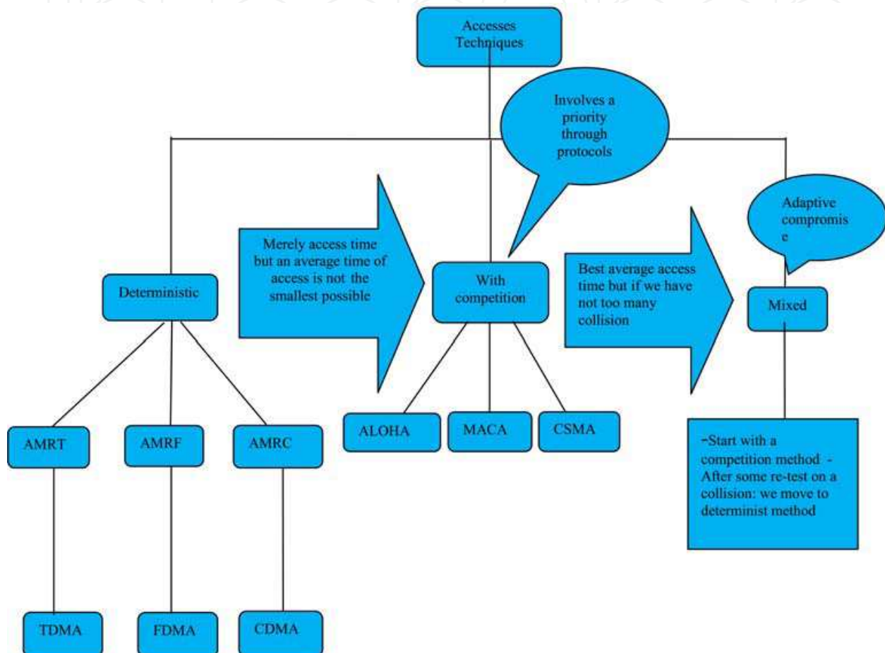
Fig. 12. Tree of accesses techniques
