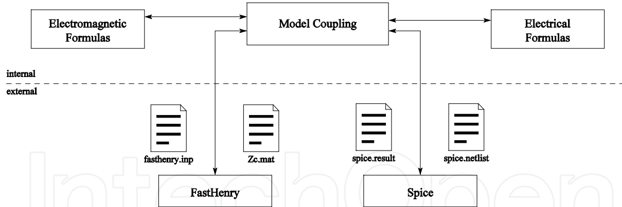
Fig. 8. Model coupling module and connected solvers
