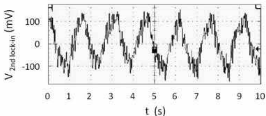
Fig. 13. Signal in the reader after the demodulation in the second lock-in amplifier.
