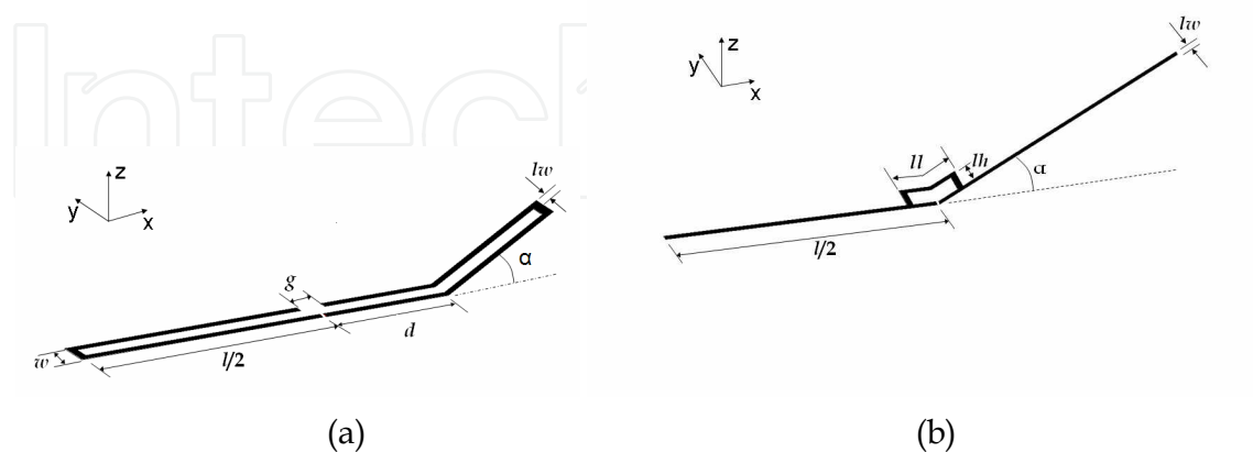
Fig. 7. An antenna will change its input impedance when distorted by bending, which is numerically simulated when bent towards the z-axis for (a) a narrowband printed folded dipole with a cut in the upper conductor for RFID impedance matching and (b) a more wideband RFID dipole.
