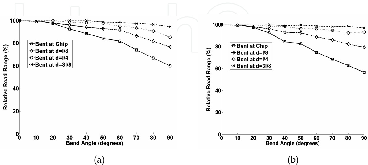
Fig. 9. Performance degradation of RFID systems for an (a) narrowband and (b) wideband dipole RFID tag antenna bent at different angles \alpha at different distances d from the structure centre.
