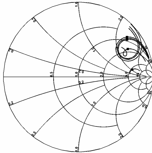
Fig. 3. Smith chart from simulations of antennas in free space and with sheet resistances 0 (PEC), 50, 100, 1000, and 5000 \text{m}\Omega/\square respectively, with the higher sheet resistances corresponding to smaller loops. Frequency spans from 500 MHz at the upper end of graphs to 1.50 GHz at the lower end. 868 MHz is marked with black dots.
