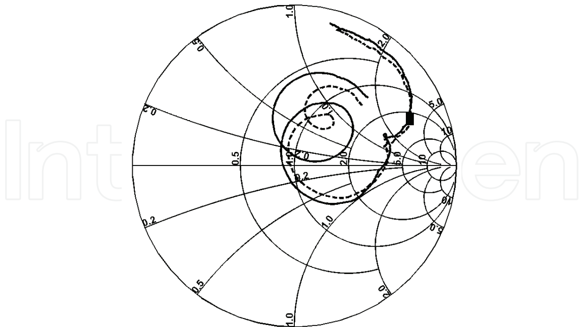
Fig. 14. Measured input impedance for the Precisia logo antenna, made from copper foil (solid line) and printed with conductive ink (dashed line). The graphs sweep from 500 to 1500 MHz and the markers on the impedance curves (the filled square) are set to 867 MHz.
