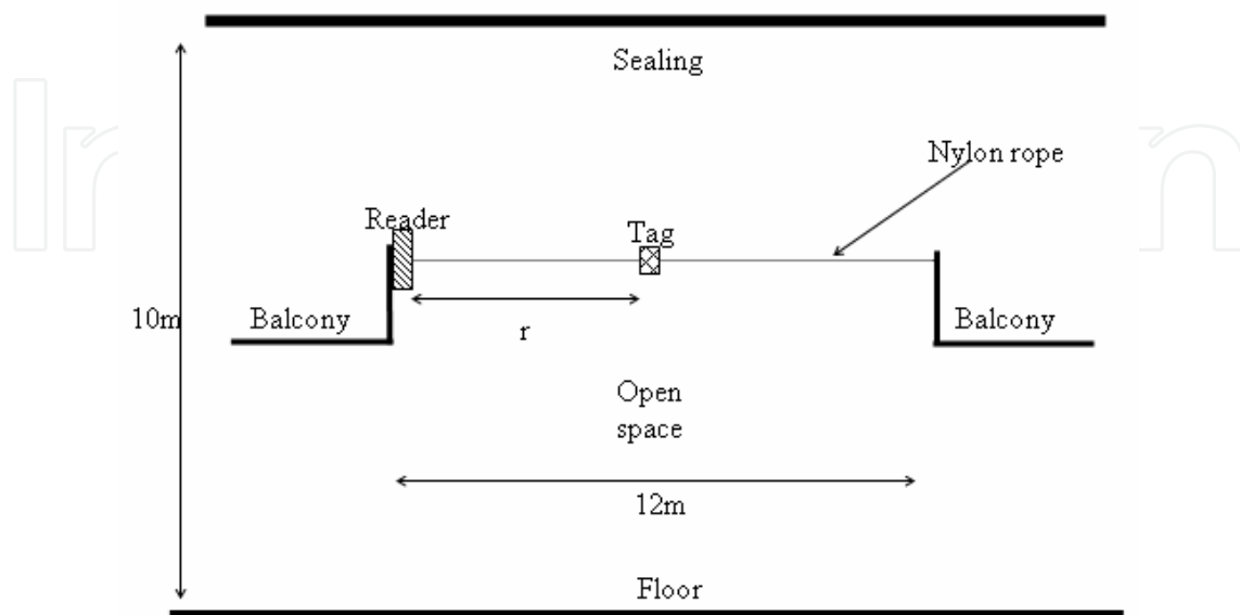
Fig. 5. Setup for determining maximum RFID read distance.
