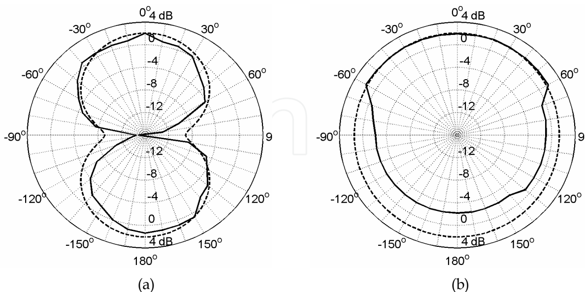
Fig. 15. Measured (solid line) and simulated (dashed line) radiation patterns for the Precisia logo antenna in (a) the xz -plane and (b) the yz -plane. Maximum directivity is about 2.0 dB, directed along the z -axis
