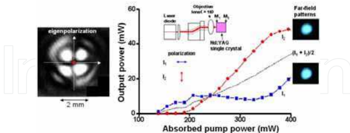
Fig. 12. Dual-polarization oscillation in the Nd:YAG single crystalline laser.
