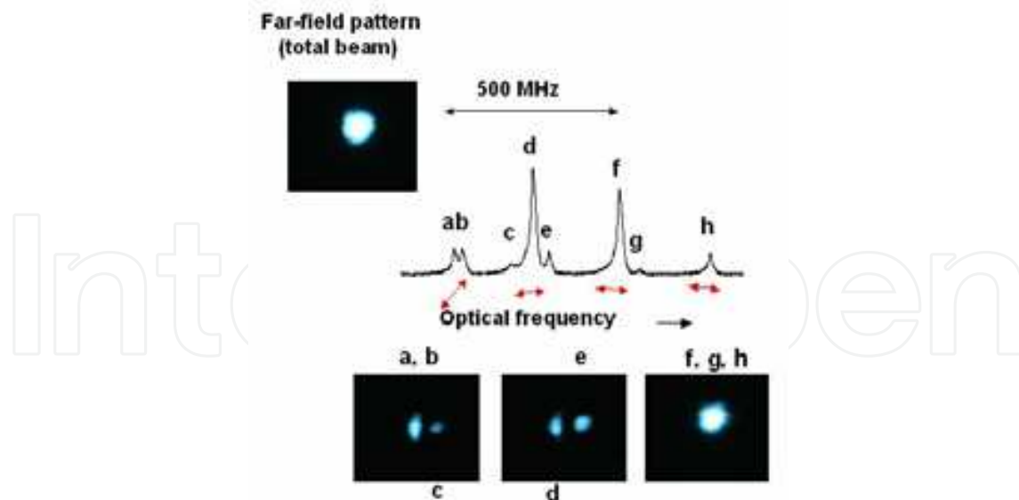
Fig. 14. Far-field patterns of total and partial beams, and their polarization states observed in the high pump-power regime.
