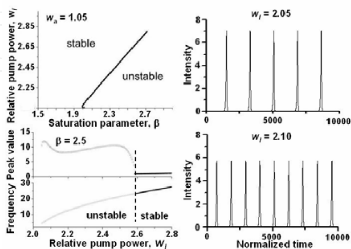
Fig. 6. Linear stability analysis and pulsation waveforms.
