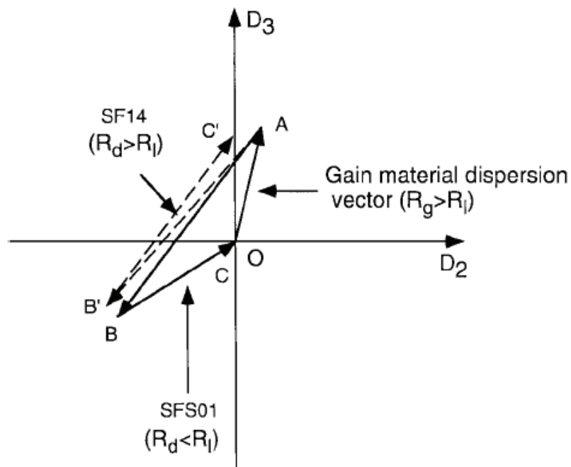
Fig. 15. Intracavity dispersion mapping for Cr:forsterite crystals
