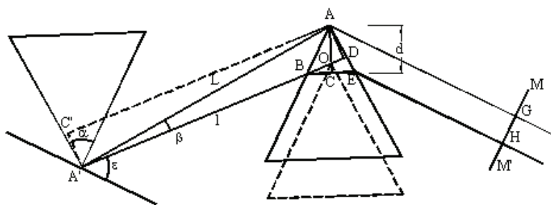
Fig. 5. A typical prism pair arrangement.
