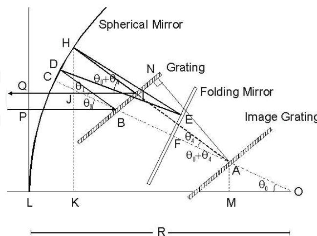
Fig. 3. Folded graing-telescope with positive dispersion
