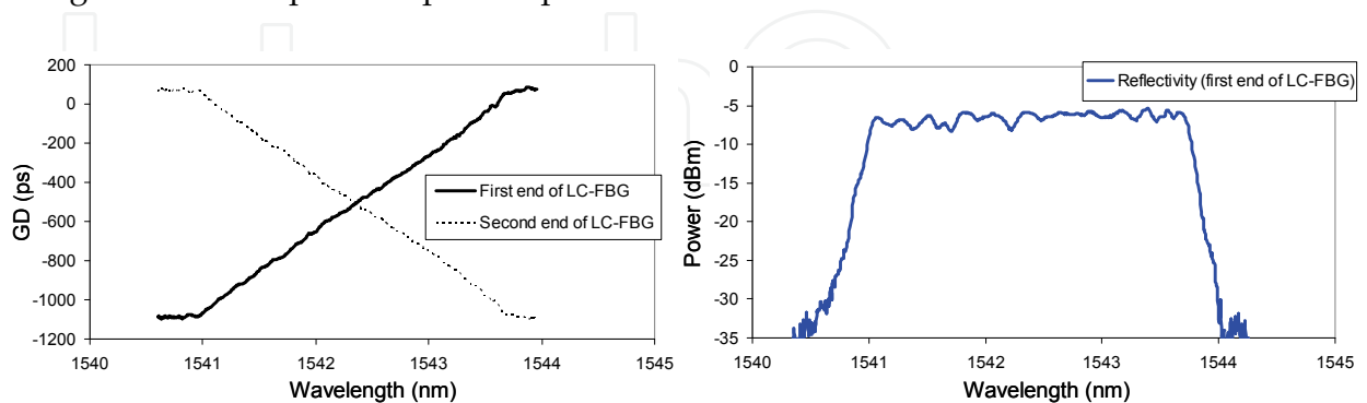
Fig. 6. Reflection behavior of the LC-FBG. (left) Group delay over the reflected bandwidth for both the ends; (right) reflected bandwidth of the first end
