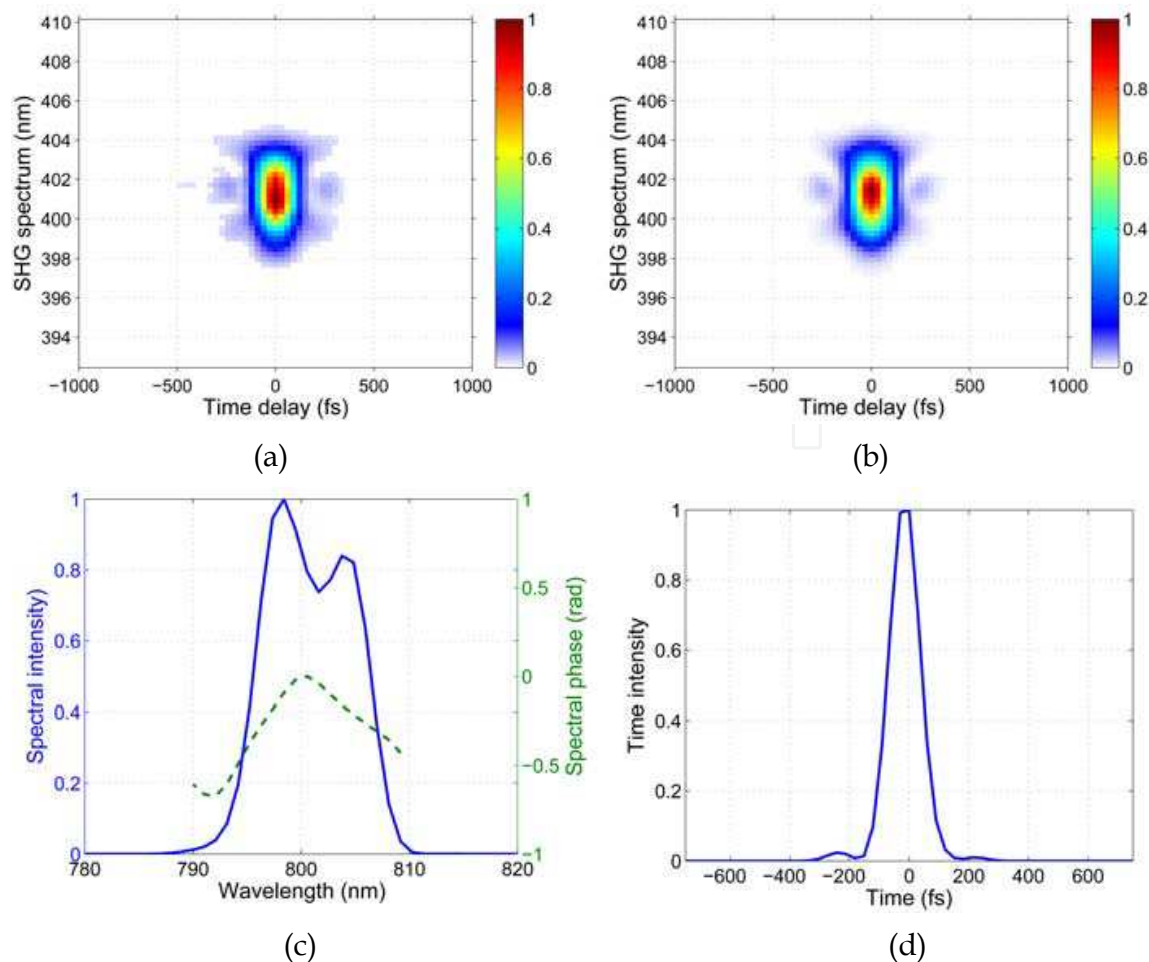
Fig. 2. a) Experimental FROG trace. b) Reconstructed FROG trace. c) Retrieved spectrum and spectral phase. d) Retrieved time intensity (123fs FWHM).
