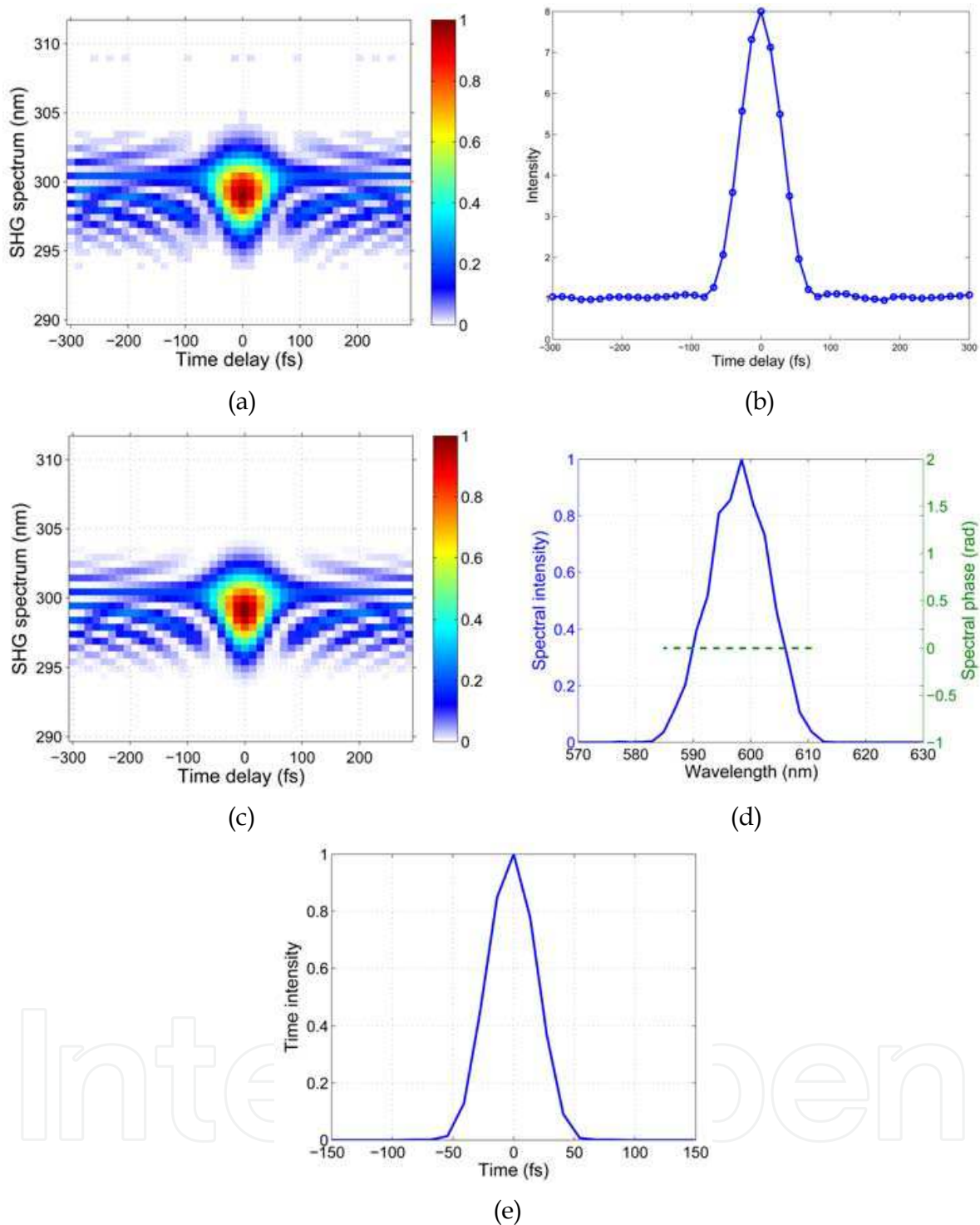
Fig. 5. a) Experimental bFROG trace. b) Experimental bFROG autocorrelation. c) Retrieved FROG trace. d) Retrieved spectral phase and intensity. e) Retrieved time intensity.
