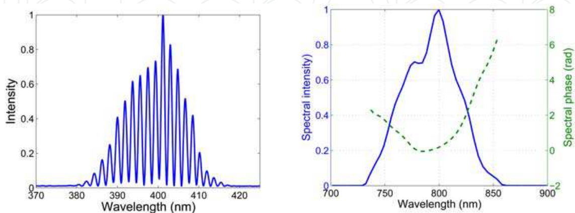
Fig. 3. a) Experimental single-shot SPIDER spectrum. b) Extracted spectral amplitude and phase. Retrieved pulse duration was 28fs FWHM.
