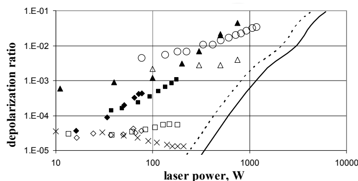
Fig. 11. Experimental plots of \gamma(P_0) (filled symbol) and \gamma_R(P_0) (open symbol) for different FIs: (Andreev et al., 2000b) (rhombs), (Nicklaus et al., 2006) (circles), (Voytovich et al., 2007) (squares, triangles), and unpublished data (crosses). Theoretical curves correspond to \gamma_R(P_0) for squares (solid) and triangles (dashed).
