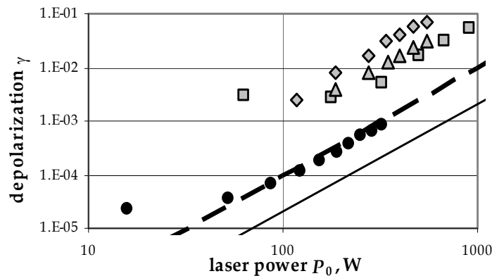
Fig. 15. \gamma as a function of P_0 for FI with B=2.1T (Mukhin et al., 2009) (circles, dashed line is theory for \alpha=2.5 \cdot 10^{-3} \text{cm}^{-1} ), and for commercial FIs (Nicklaus et al., 2006) produced by Litton (rhombuses), Linos (triangles), and EOT (squares). Solid line is theory for FI with B=2.5T and \alpha=1.5 \cdot 10^{-3} \text{cm}^{-1} .
