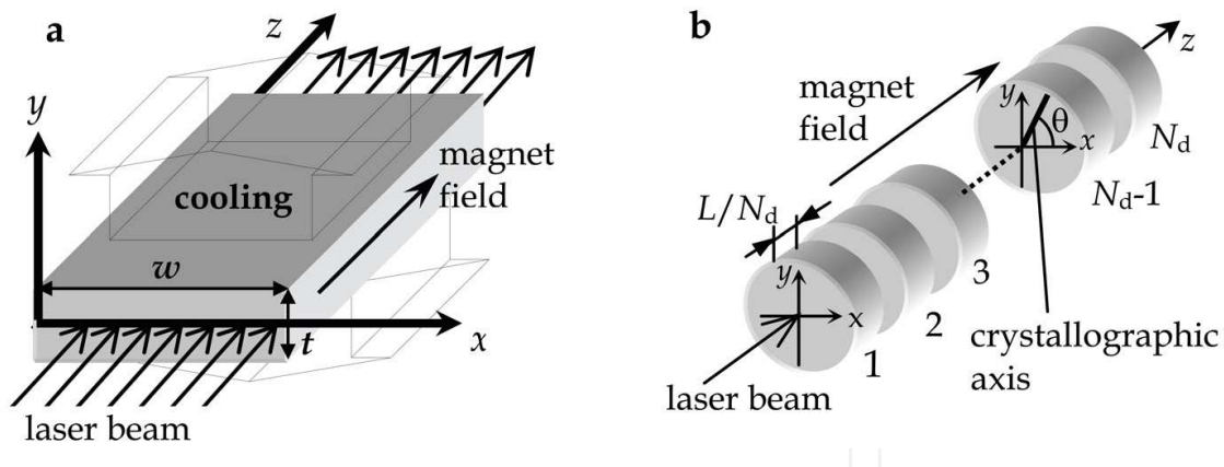
Fig. 16. Use of slabs (a) or discs (b) in Faraday isolators.
