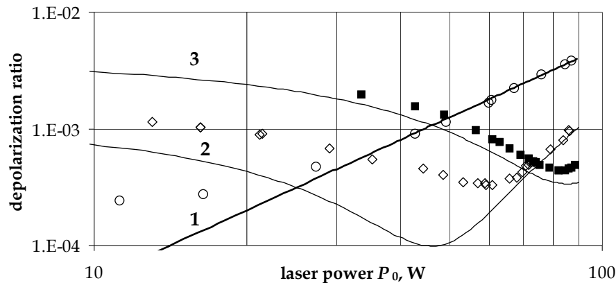
Fig. 8. Depolarization ratio in traditional FI design \gamma(P_0) (curve 1, circles) and design in Fig. 7 \gamma_q(P_0) at f=125\text{mm} (curve 2, rhombs) and f=88\text{mm} (curve 3, squares) (Andreev et al., 2002).
