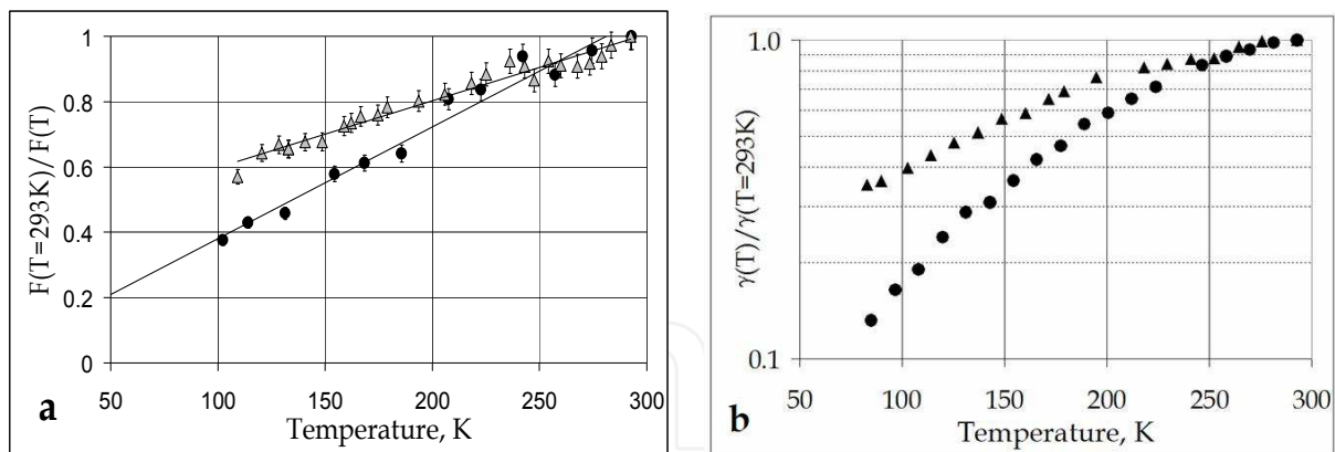
Fig. 12. Temperature dependence of the focal length of thermal lens F (a) and depolarization \gamma (b) in the TGG with the [001] orientation (circles, F(T=293\text{K})=191\text{cm} , \gamma(T=293\text{K})=5.2 \cdot 10^{-3} ) and in glass MOC-04 (triangles, F(T=293\text{K})=581\text{cm} , \gamma(T=293\text{K})=5.1 \cdot 10^{-3} ).
