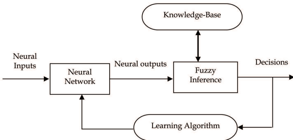
Fig. 1. Neural fuzzy system (Fuller, 2000).
