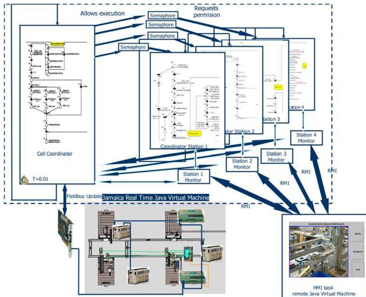
Fig. 6. Control architecture
