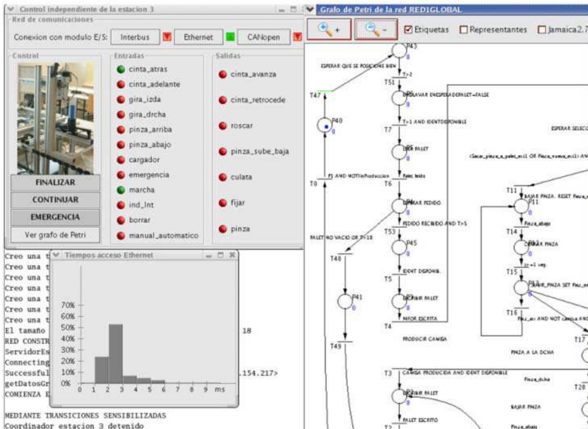
Fig. 8. Human Machine Interface.
