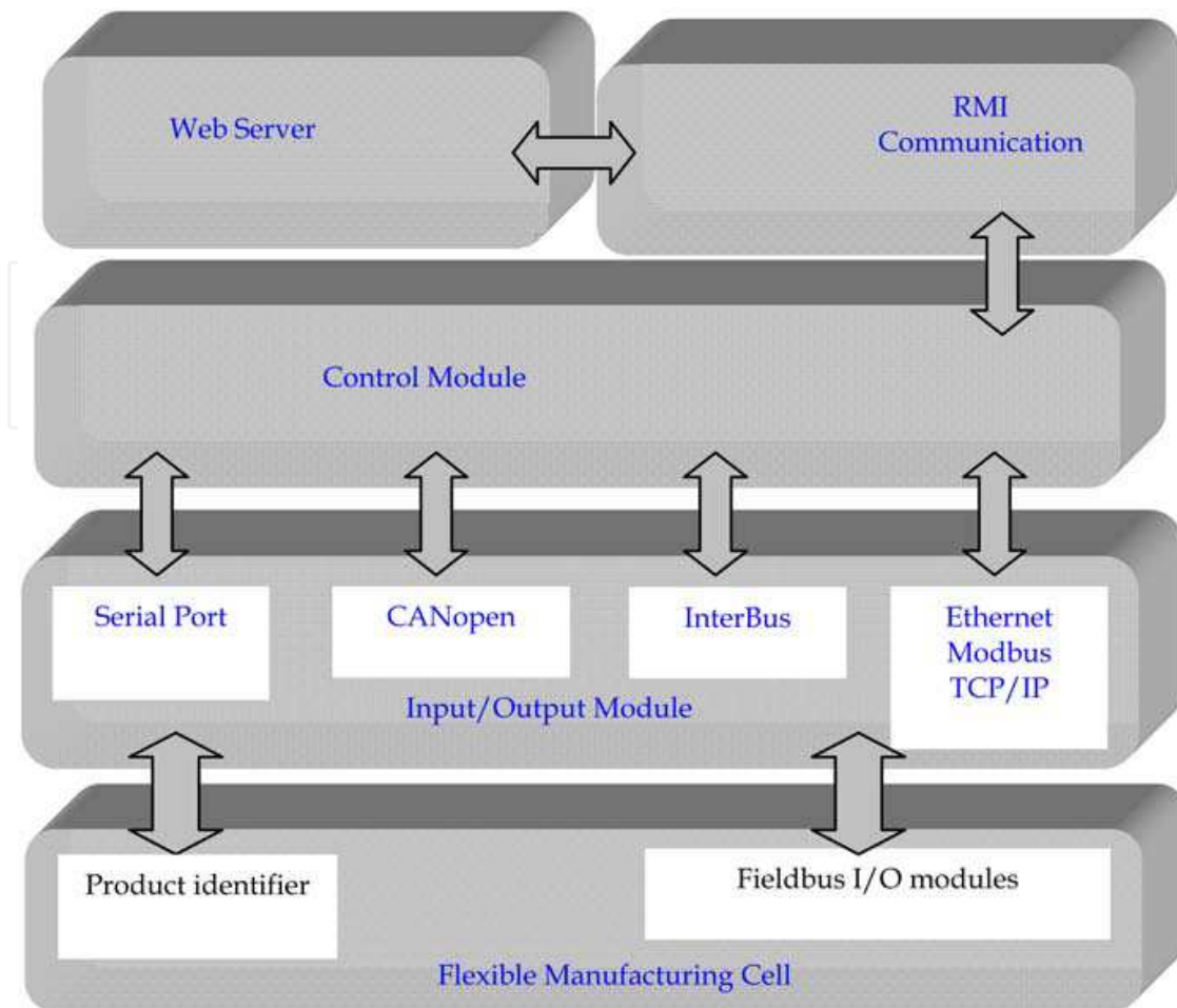
Fig. 1. Java based Programmable Logic Controller.
