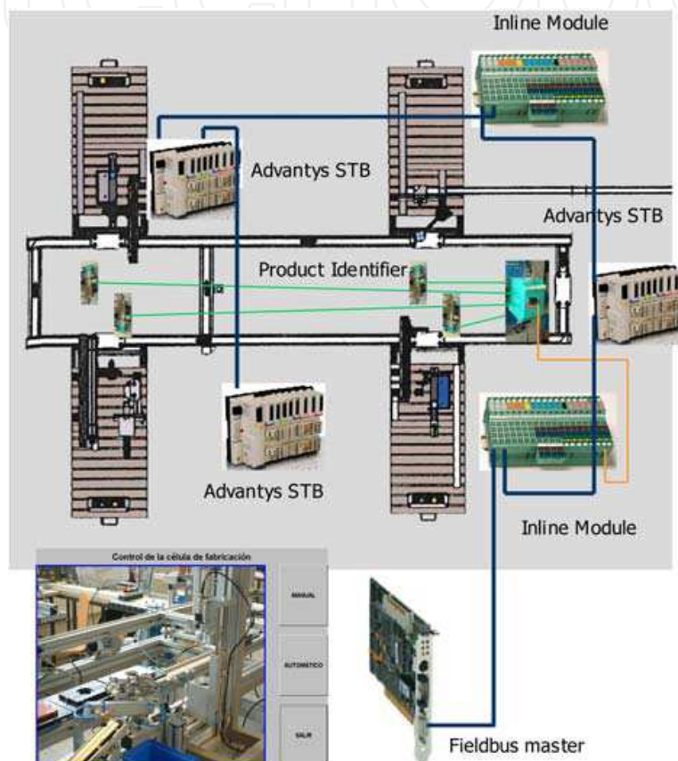
Fig. 5. Fieldbus and Product Identifier
