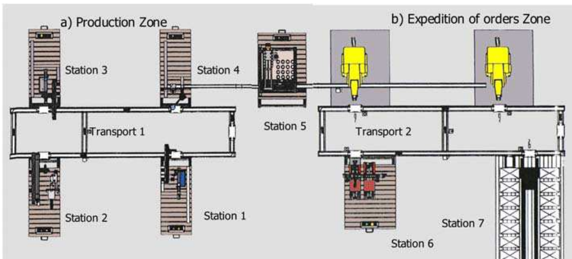
Fig. 4. Flexible manufacturing cell.
