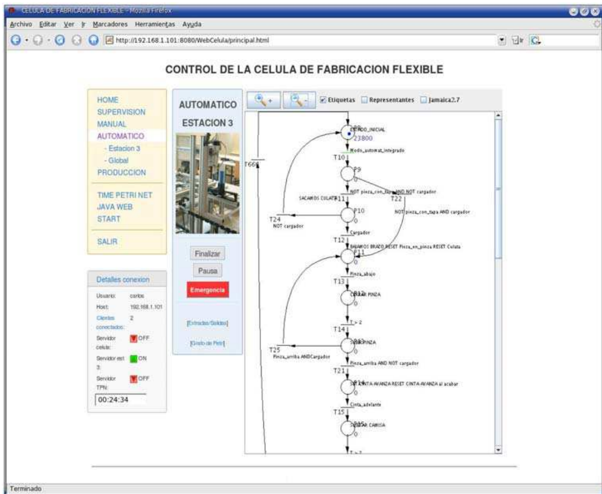
Fig. 10. Petri Net Visualization in a web browser.
