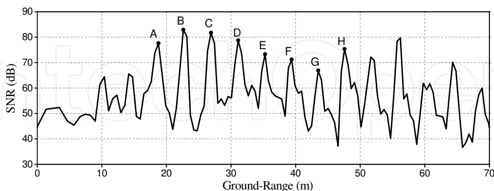
Fig. 16. Ground-Range profile in load condition LC1
