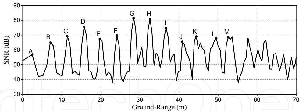
Fig. 19. Ground-Range profile in load condition LC2
