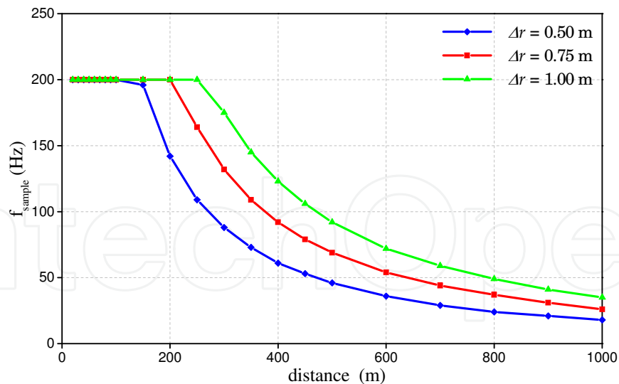
Fig. 6. Sampling rate vs. maximum distance for three different values of \Delta r
