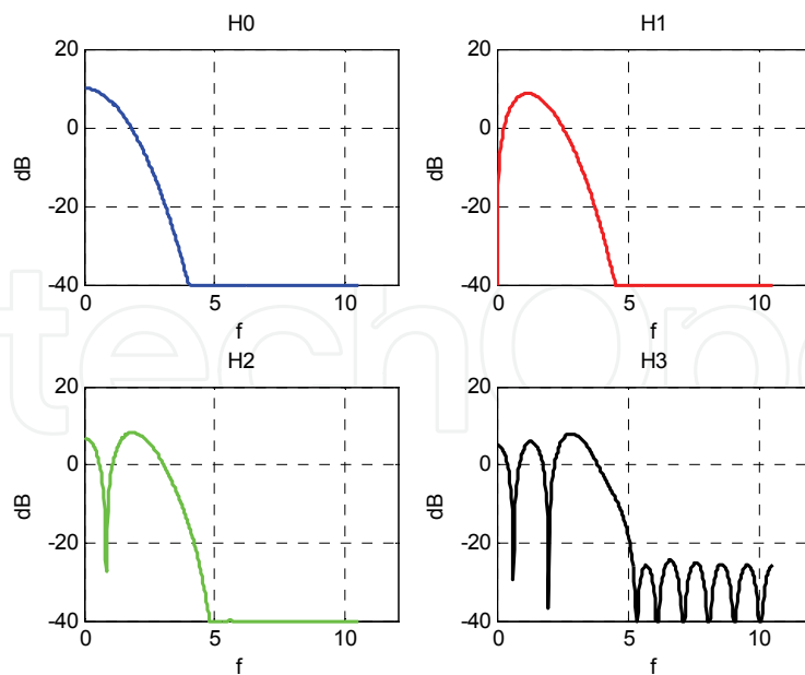
Fig. 8. Spectral representation for Hermite functions of orders n = 0 to 3.
