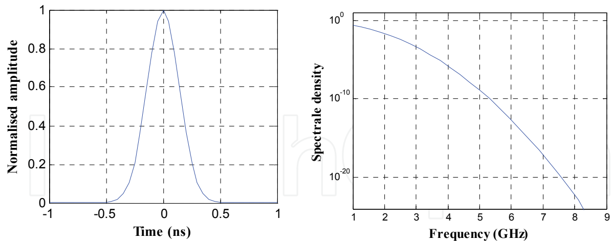
Fig. 1. Gaussian pulse time and spectral representations.
