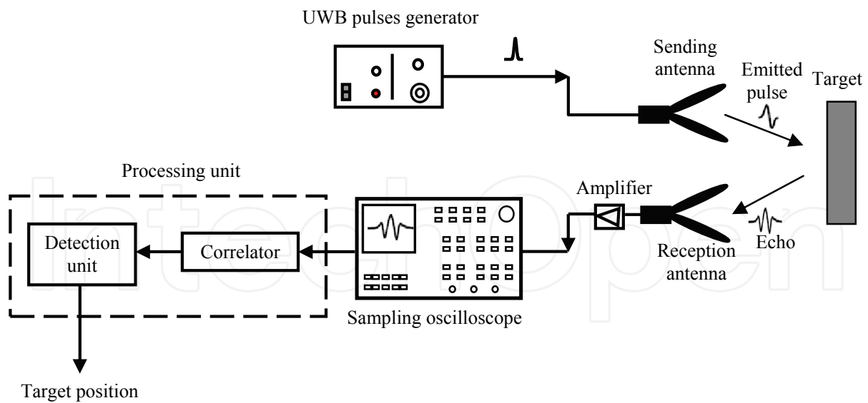
Fig. 3. The radar based on UWB pulses.
