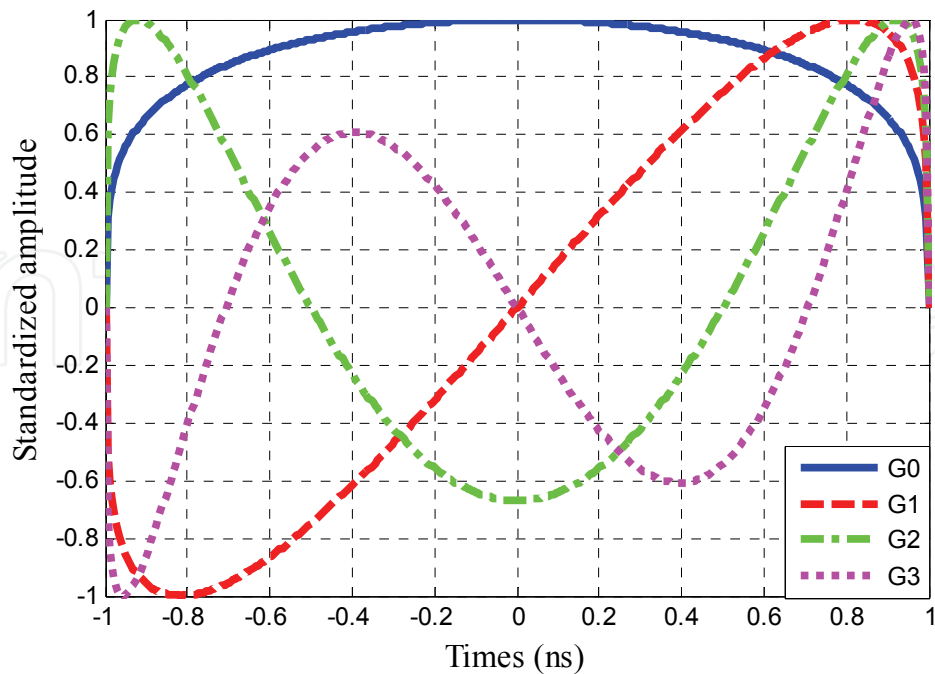
Fig. 5. Modified Gegenbauer functions of orders n = 0, 1, 2 and 3 .
