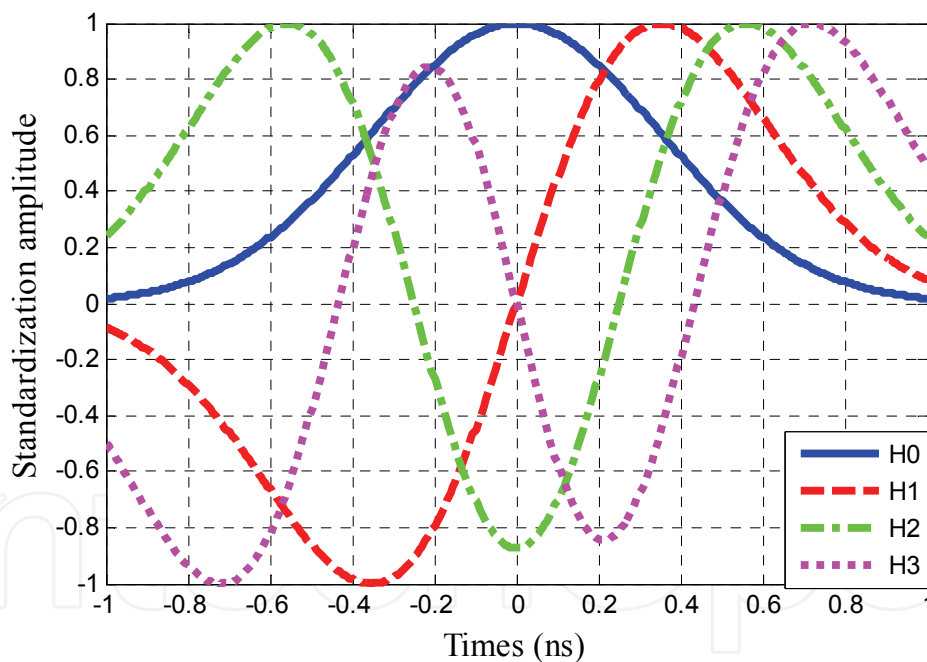
Fig. 7. Hermite functions, orders n = 0 to 3.
