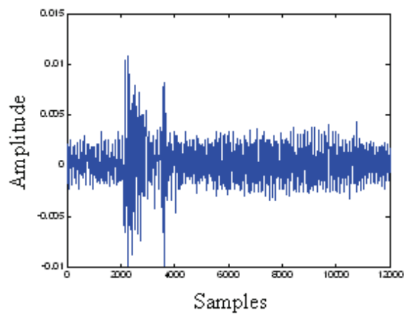
Fig. 19. Reflected signal by pedestrian placed at 2 m.
