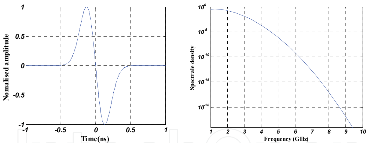
Fig. 2. Monocycle pulse time and frequency representations.
