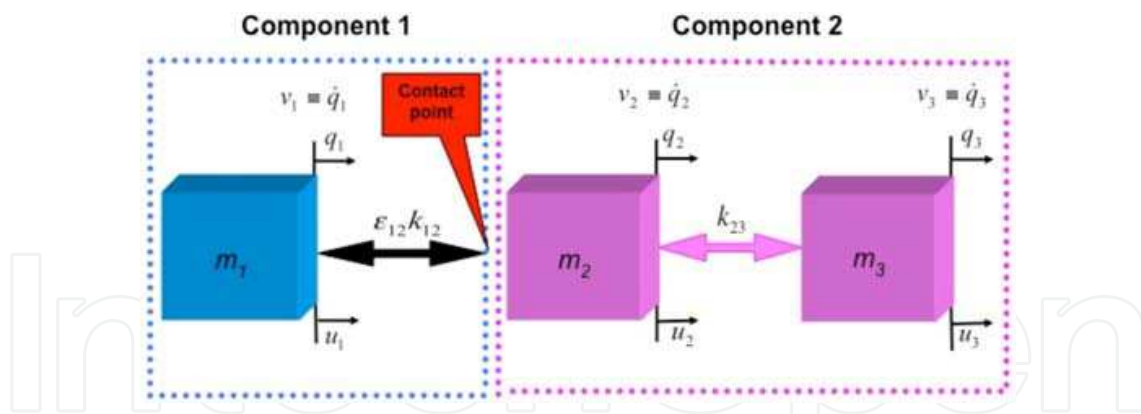
Fig. 3. Ex. 1: A two component flexible structure Evolving System.
