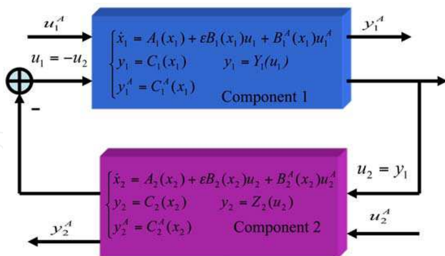
Fig. 8. Admittance-Impedance feedback connection of two nonlinear subsystems.
