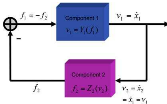
Fig. 2. Admittance-impedance feedback connection of two components.
