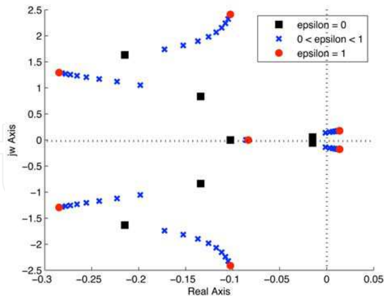
Fig. 4. Closed-loop poles of Ex. 1.
