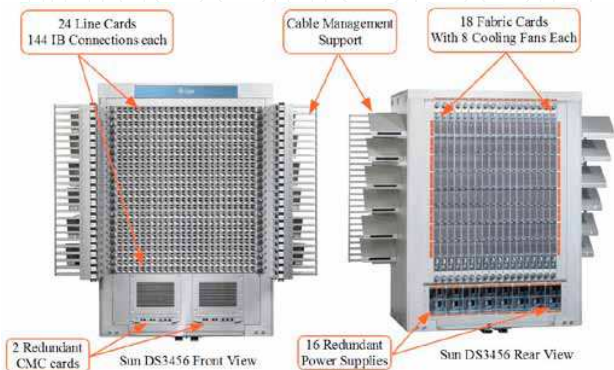
Fig. 1. DS3456 Physical View
