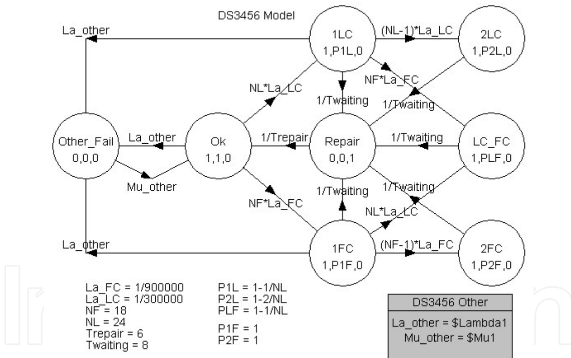
Fig. 3. Top level Markov model
