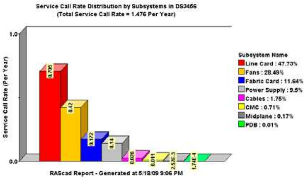
Fig. 5. Distribution of service events
