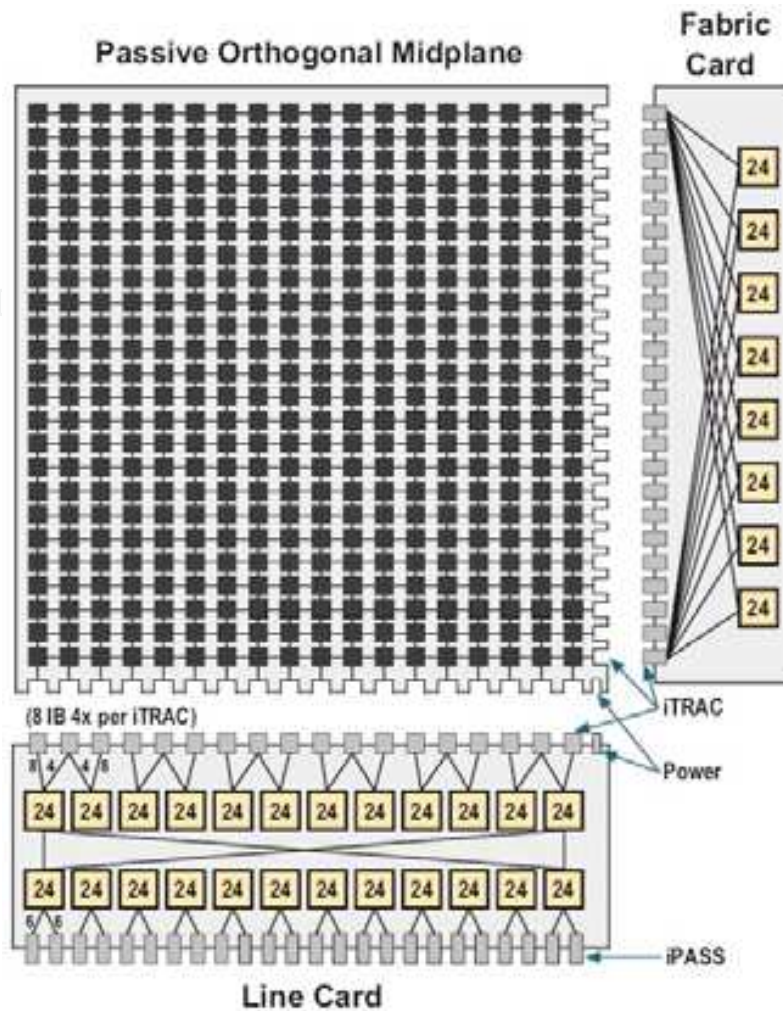
Fig. 2. DS3456 Internal Connectivity
