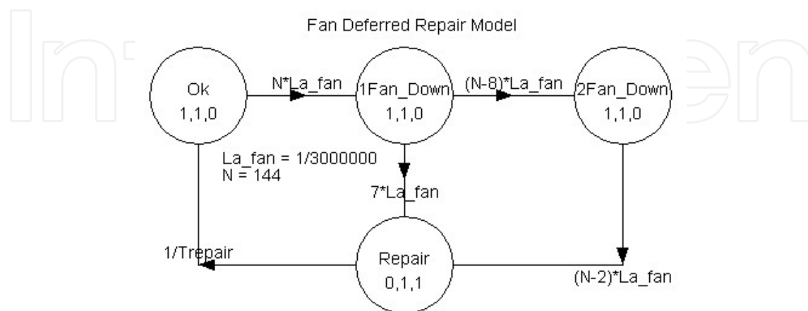
Fig. 6. Deferred repair model for fans
