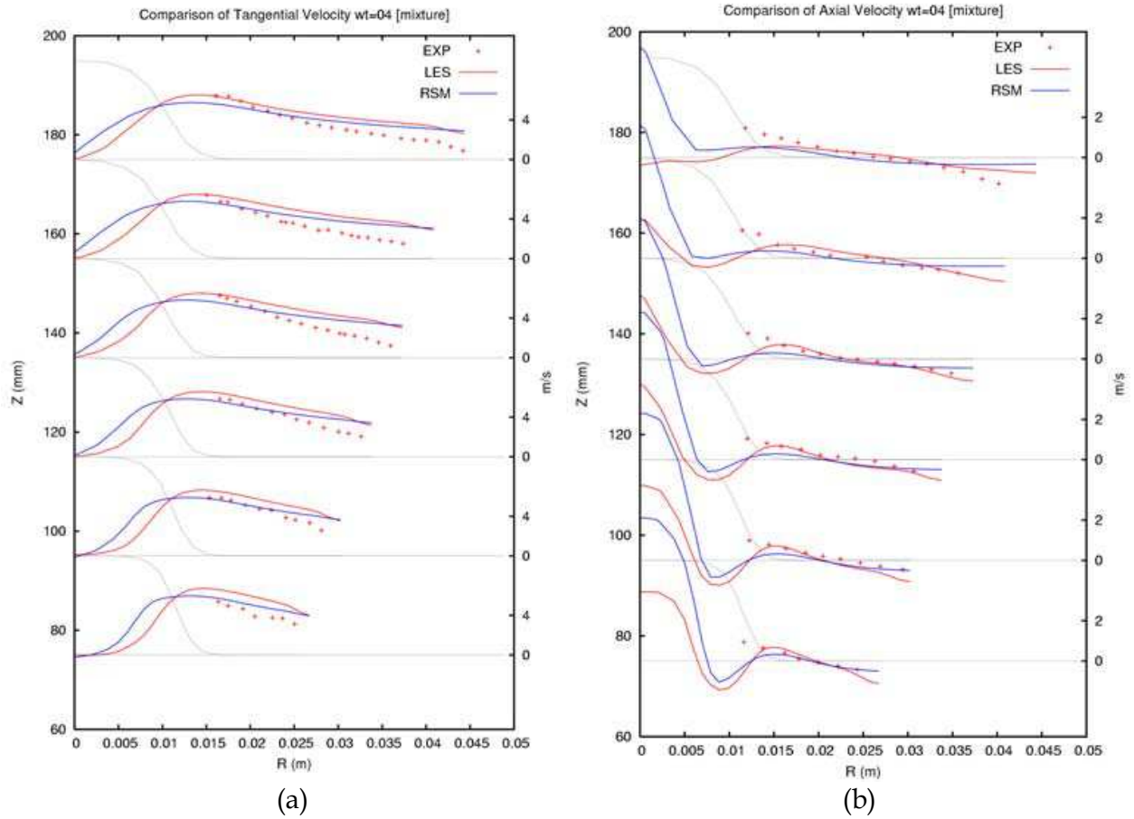
Fig. 2. Comparison of predicted (a) tangential velocity field, (b) axial velocity field with experimental data (Fanglu and Wenzhen (1987))
