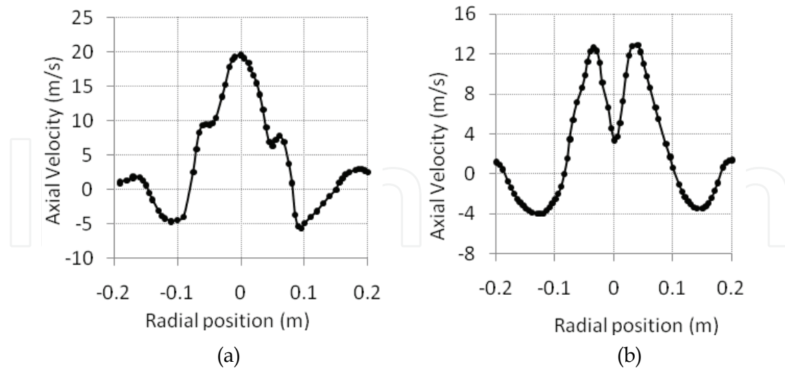
Fig. 4. Typical axial velocity profile (a) V pattern and (b) W pattern (Adapted from Harasek et al. 2008)
