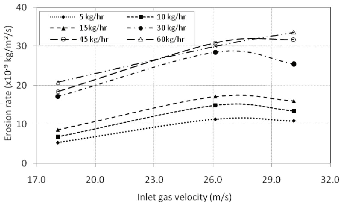
Fig. 14. Comparison of erosion rate with various gas and particle flow rate
