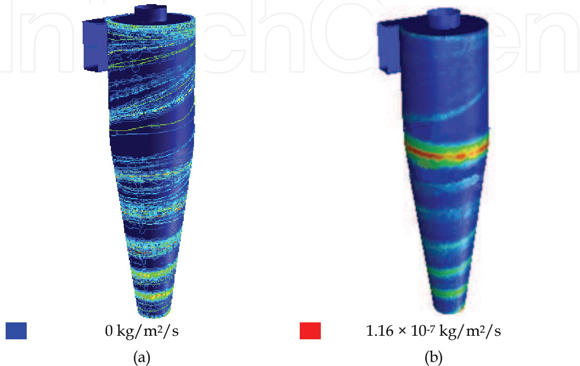
Fig. 12. (a) Contours of erosion (a) with uniform catalyst size (b) Rosin-Rammler PSD
