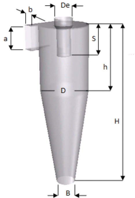
Fig. 1. Typical design of cyclone separator
