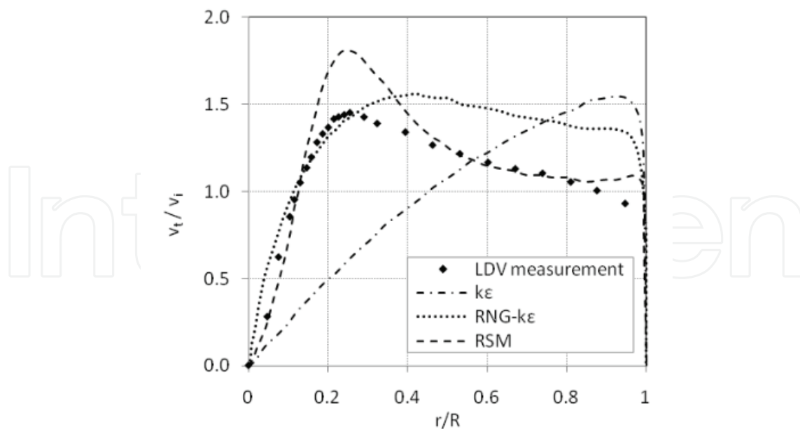
Fig. 3. Comparison of tangential velocity profiles (Adapted from Hoekstra et al., 1999)
