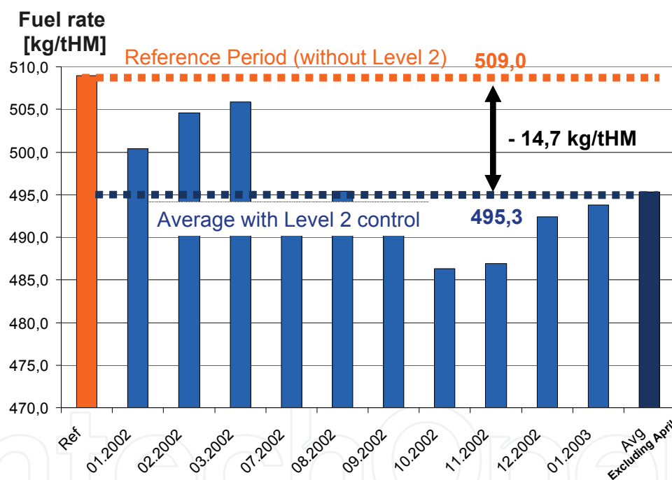
Fig. 5. Fuel Rate Savings Over Time
