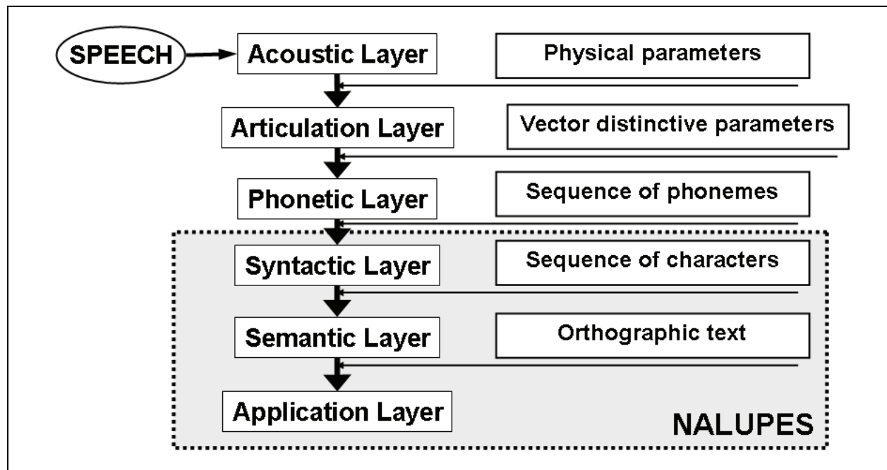
Fig. 7. Multilayer speech recognition process.
