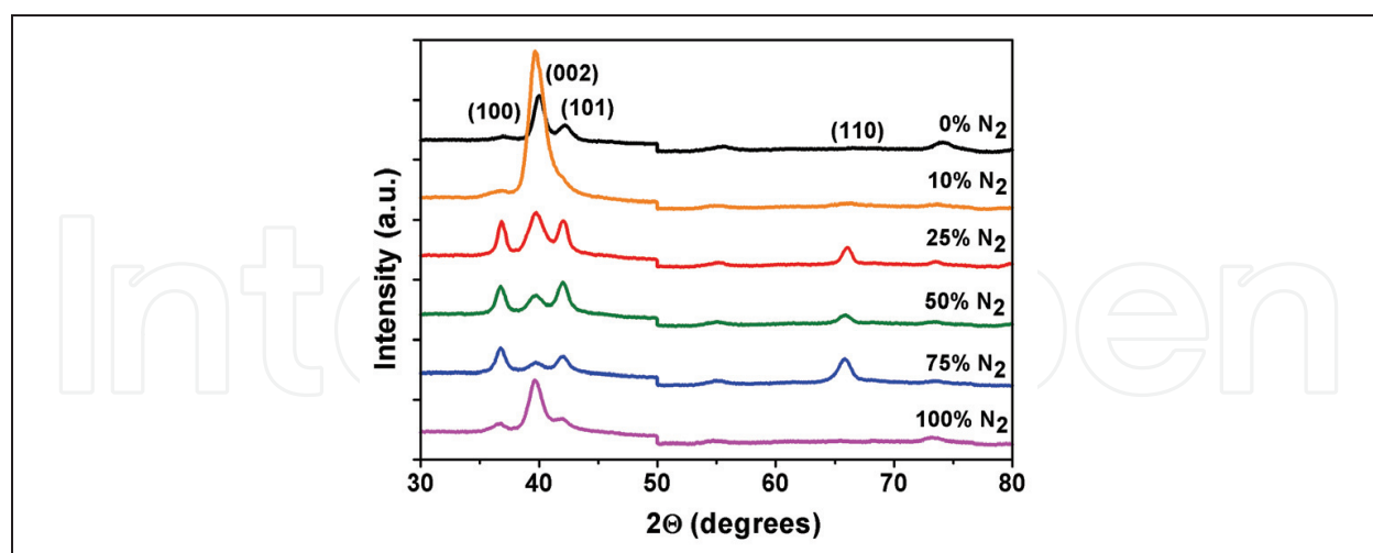
Fig. 3. X-ray diffraction patterns of ZnO:N deposited on Corning glass 7059 substrates as a function of nitrogen percentage in the working gas
