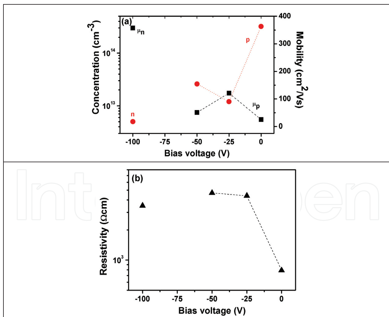
Fig. 10. Effect of the bias voltage on (a) the carrier concentration and mobility and (b) resistivity, for ZnO:N deposited on Corning glass 7059 substrates
