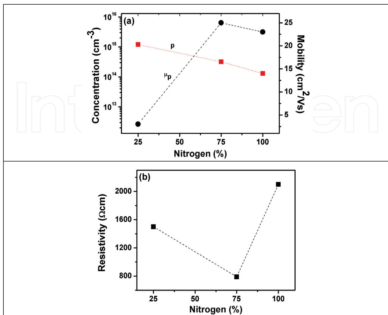
Fig. 8. Effect of the N 2 content on (a) the carrier concentration and mobility, and (b) resistivity for ZnO:N deposited on Corning glass 7059 substrates
