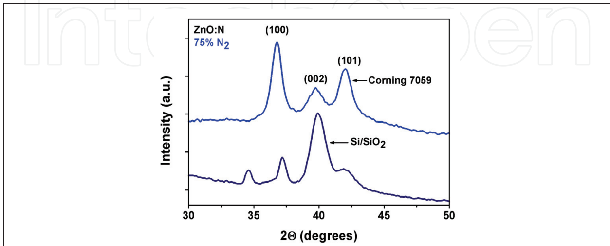
Fig. 6. X-ray diffraction patterns of ZnO:N deposited on Corning glass 7059 and Si/SiO 2 substrates at 75 % N_2 content in the working gas
