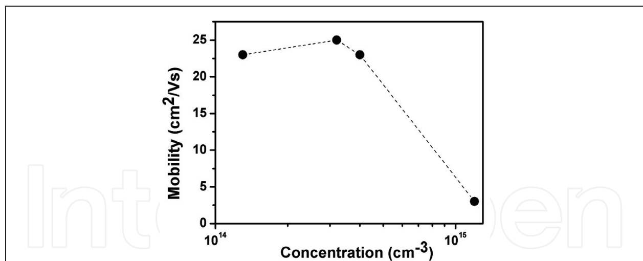
Fig. 9. Mobility of ZnO:N films as a function of the carrier concentration
