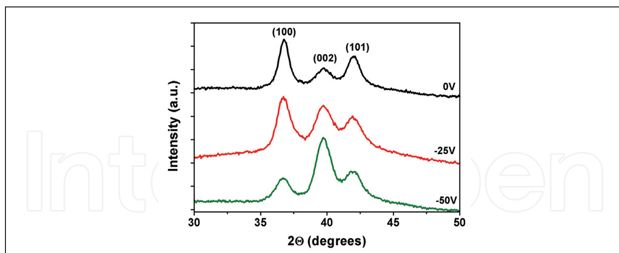
Fig. 4. XRD patterns of ZnO:N thin films deposited on Corning glass 7059 substrates at 75 % N_2 content as a function of the bias voltages
