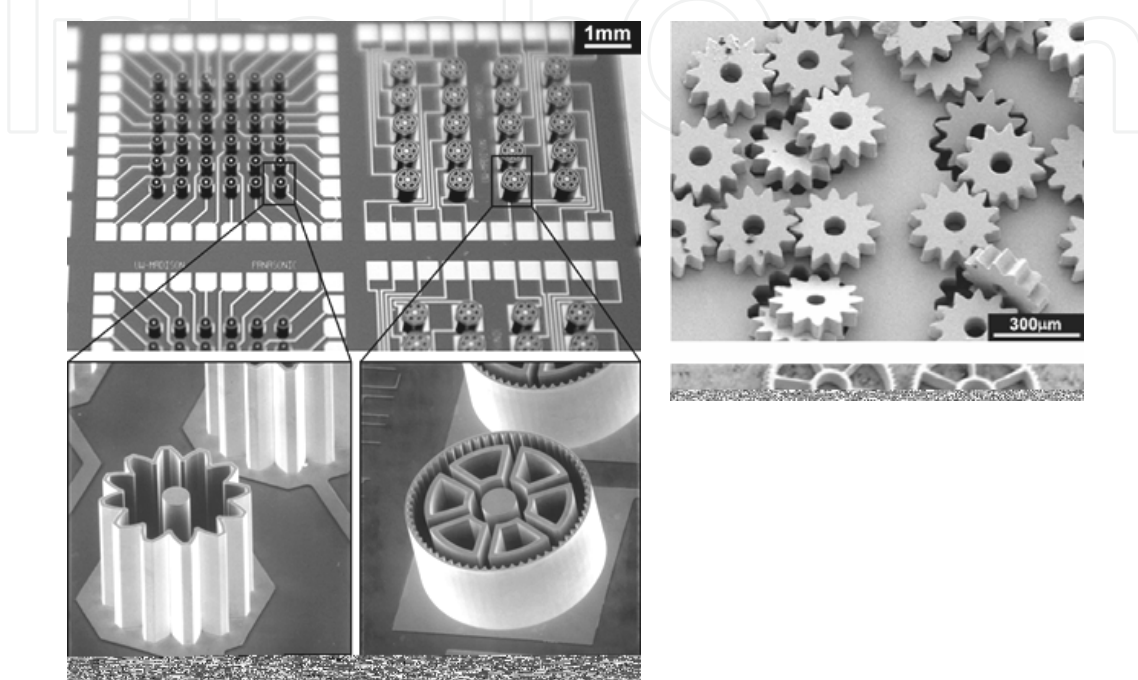
Fig. 10. (a: left) Partitioned copper electrode arrays with interconnect; (b: right) super-hard alloy gears batch produced using the arrays (Takahata & Gianchandani, 2002) © 2002 IEEE.
