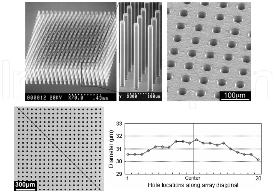
Fig. 7. (a: upper left) A 20×20 array of LIGA fabricated copper electrodes; (b: upper right) through-holes batch machined in 50- \mu\text{m} -thick stainless steel using the array; (c: lower) a top-view image of the machined hole array, and measured variation of hole diameter along the array diagonal shown in the image (Takahata & Gianchandani, 2002) © 2002 IEEE.
