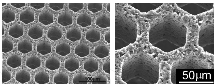
Fig. 8. Graphite honeycomb microstructures (hexagonal pitch of 70 \mu\text{m} and wall thickness of 16 \mu\text{m} ) formed by batch-mode \mu\text{EDM} (Takahata & Gianchandani, 2002) © 2002 IEEE.
