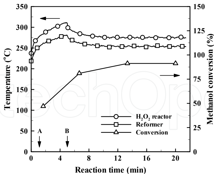
Fig. 13. Simultaneous operation of the micro reformer with hydrogen peroxide heat source
