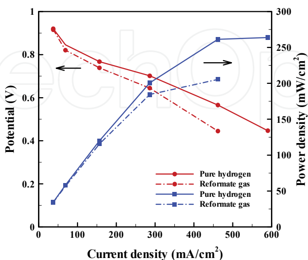
Fig. 21. Performance curve of MEMS fuel cell system
