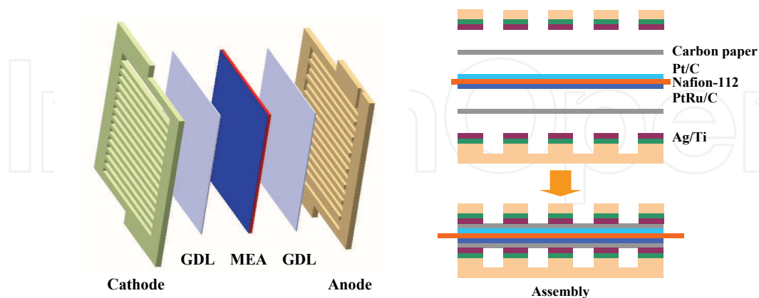
Fig. 18. Structure and fabrication process of MEMS fuel cell
