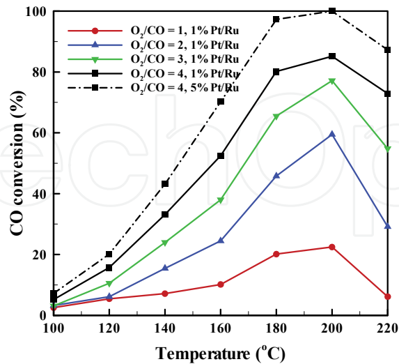
Fig. 17. Conversion of carbon monoxide of PROX microreactor
