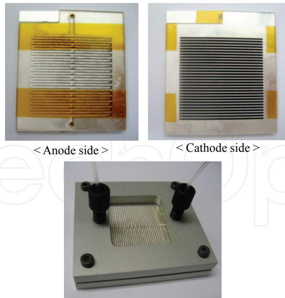
Fig. 19. Fabricated results of the micro fuel cell
