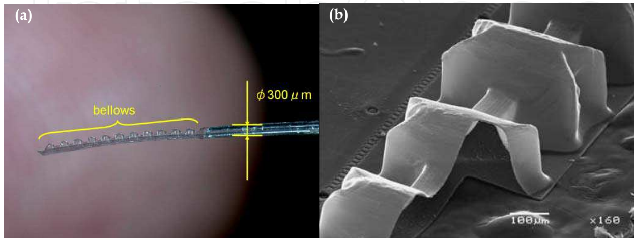
Fig. 10. (a) Completed pressure-driven micro active catheter \phi 300 \mu m. (b) SEM image of the bellows cut at the middle to show the cross-section and the inner structure.
