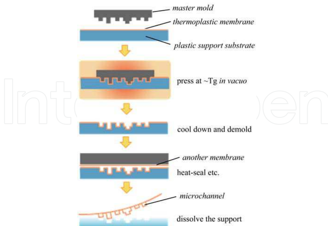
Fig. 2. Flowchart of the MeME process
