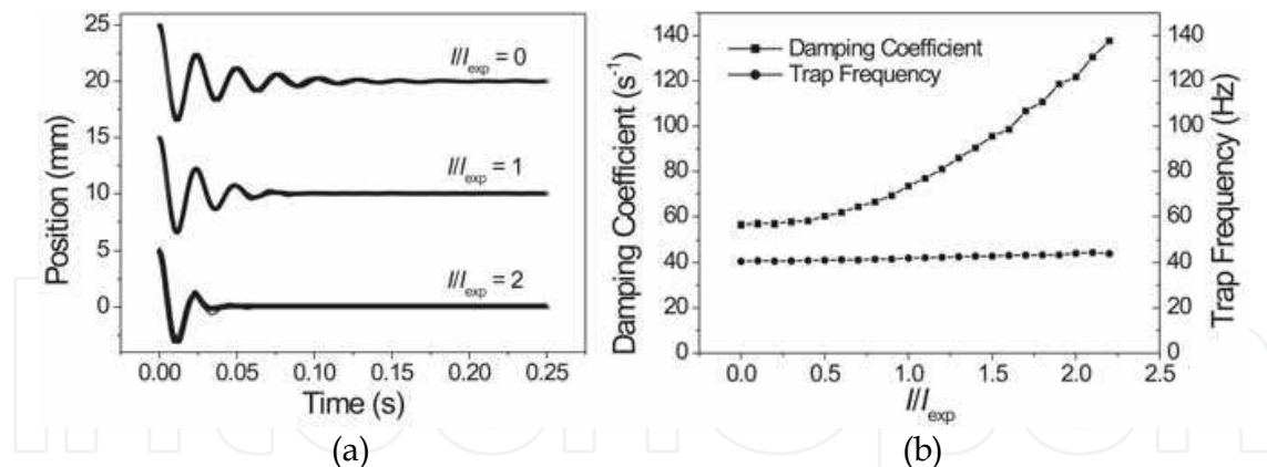
Fig. 15. The Monte-Carlo simulation results. (a) The averaged trajectories for 1000 atoms together with the fitted curves obtained from Eq. (17). (b) The damping coefficient (filled square) and the trap frequency (filled circle) as a function of the laser intensity.
