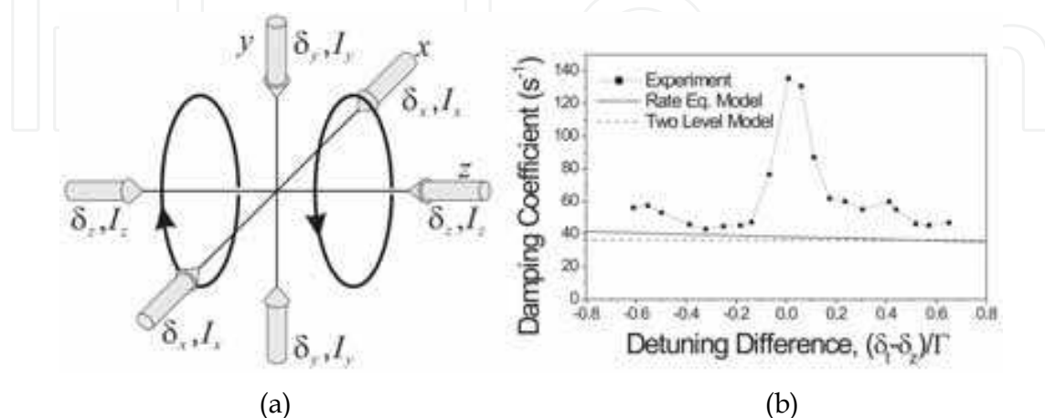
Fig. 16. (a) Schematic of the asymmetric magneto-optical trap. (b) Measured damping coefficients versus normalized laser-detuning differences.
