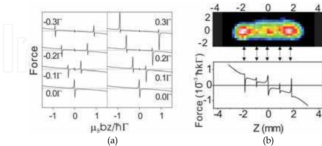
Fig. 19. (a) Calculated forces F(z, \nu = 0) for various detuning differences. The maximum forces at 0.3 \Gamma corresponds to 5 \times 10^{-3} \hbar k \Gamma . Here \delta_z = -2.7\Gamma , I_z = 0.11 \text{ mW/cm}^2 , and I_t = 5.6I_z . (b) Five SDTs, including two weak SDTs midway between the two side SDTs and the central one, for \delta_t - \delta_z = -0.24\Gamma .
