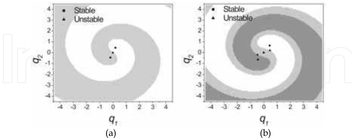
Fig. 2. The stability regions for the frequency Region I (a) and Region II (b).
