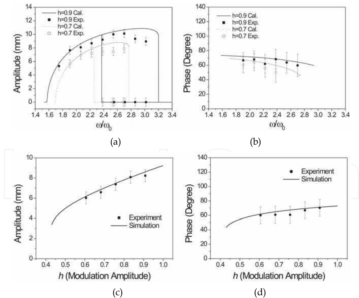
Fig. 5. The dependence of amplitude (a) [(c)] and phase (b) [(d)] of limit cycles on the modulation frequency [amplitude].
