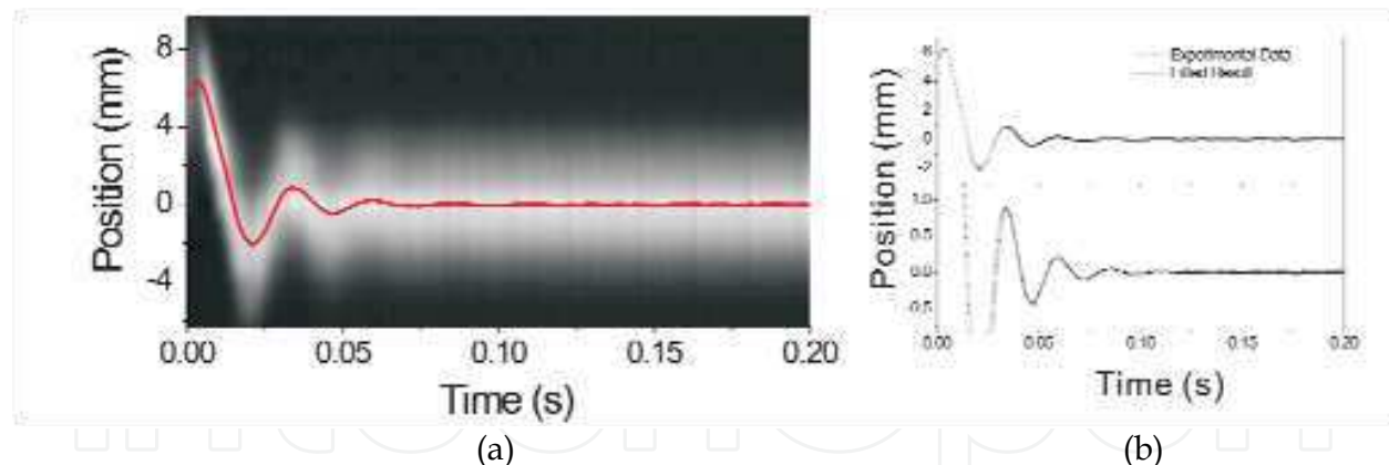
Fig. 12. (a) The contour plot of the signals showing a typical oscillating motion of atomic cloud. (b) The same curve as in (a) and the fitted curve obtained by Eq. (17). The detailed plot after one period is shown in the lower panel.
