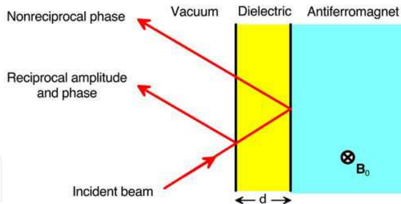
Fig. 19. Use of a dielectric layer for investigating nonreciprocal phase on reflection off an antiferromagnet.
