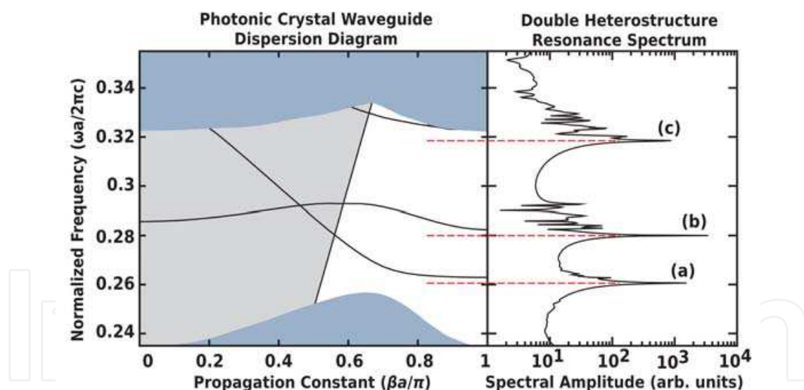
Fig. 7. Left: photonic crystal waveguide dispersion diagram. Black lines correspond to the photonic crystal waveguide dispersion bands. Blue regions denote photonic crystal cladding modes. The gray region denotes the light cone projection. Right: photonic crystal double heterostructure resonant spectrum. Dashed lines illustrate correspondance between heterostructure bound state frequencies and waveguide dispersion extrema.
