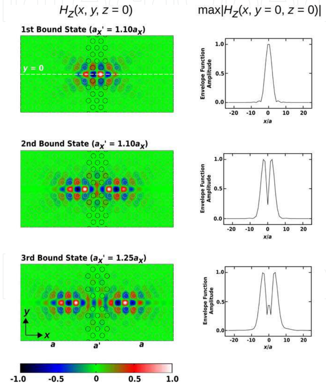
Fig. 10. Left: H_z(x, y, z = 0) field distributions for the first, second and third order bound states. Right: field envelopes extracted from |H_z(x, y = 0, z = 0)| .
