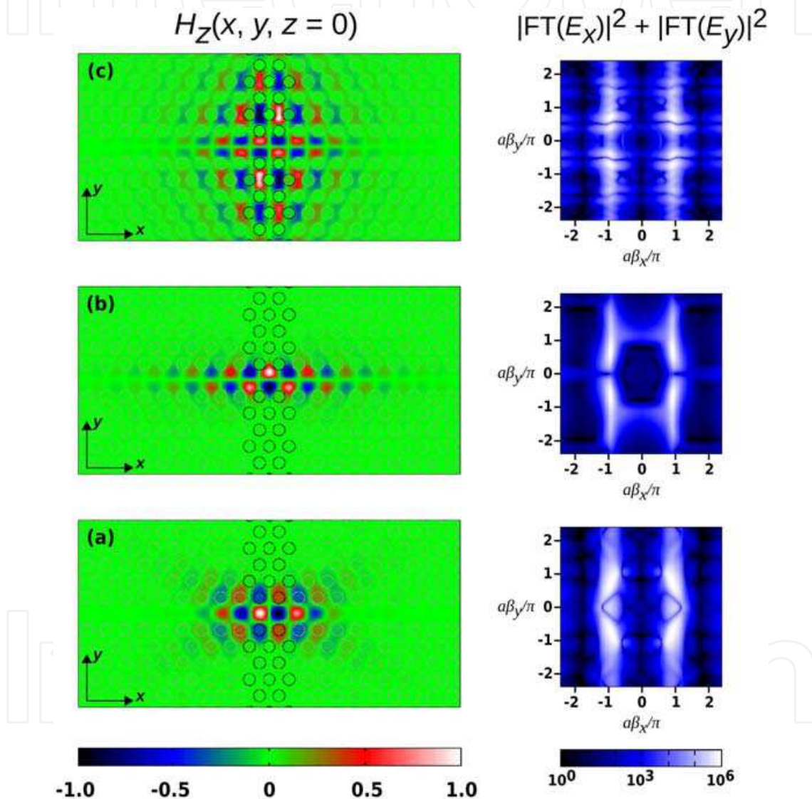
Fig. 8. Left: H_z(x, y, z = 0) for the three modes summarized in Table 1. Right: spatial Fourier transform \log(|FT(E_x)|^2 + |FT(E_y)|^2) of each mode illustrating the distribution of spatial wavevectors making up the different resonant modes.
