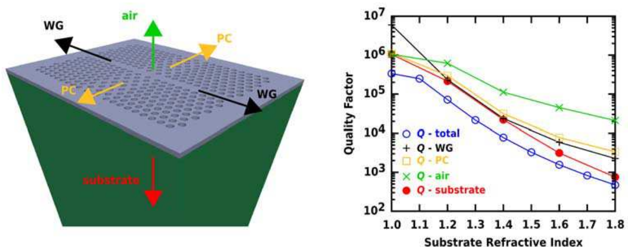
Fig. 13. (a) Depiction of a photonic crystal heterostructure cavity bonded or grown on a lower substrate. Radiation directions are indicated. (b) Q factor versus substrate refractive index for the total Q factor as well as the directional Q factors.
