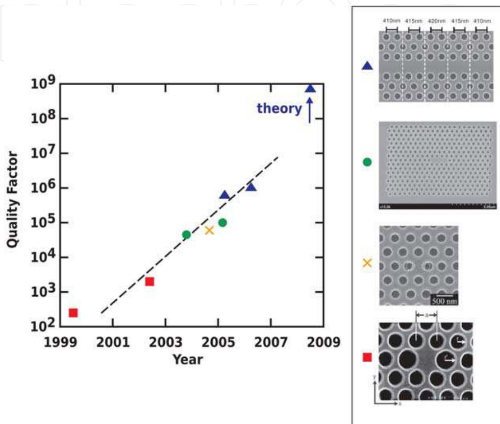
Fig. 5. Quality factor for different two-dimensional photonic crystal cavities as a function of time. Data points and figures come from (Painter et al., 1999; Ryu et al., 2002; Akaahane et al., 2003; Zhang & Qiu, 2004; Nozaki & Baba, 2006; Akaahane et al., 2005; Song et al., 2005; Asano et al., 2006; Tanaka et al., 2008)
