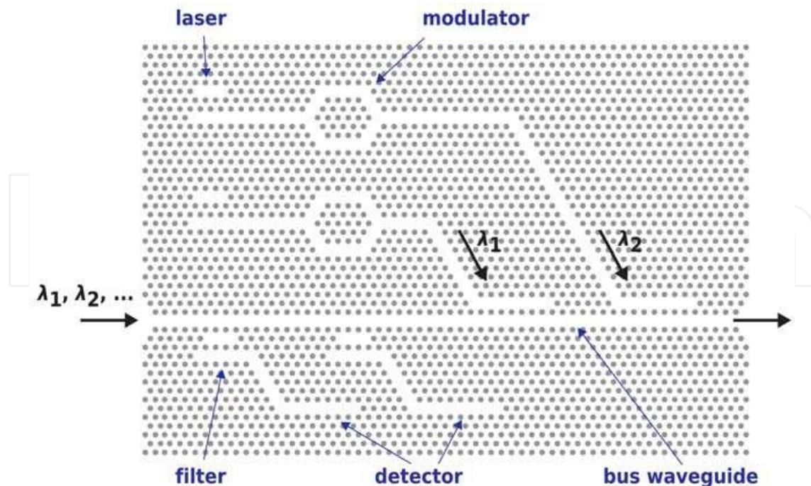
Fig. 4. Schematic diagram depicting a simple photonic crystal based photonic integrated circuit.
