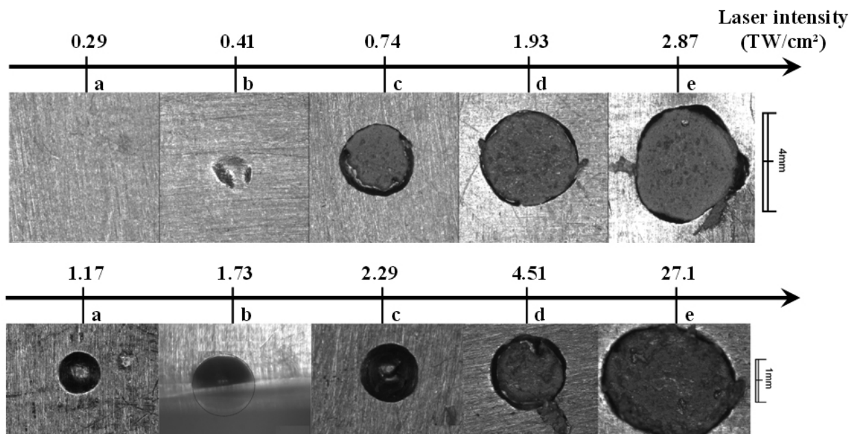
Fig. 8. Overview of the free surface in 1 mm-thick aluminium targets recovered from laser shocks of increasing intensities with two different laser spot diameters : D = 4 mm, L/D = 0.25 (top) ; D = 1 mm, L/D = 1 (bottom).
