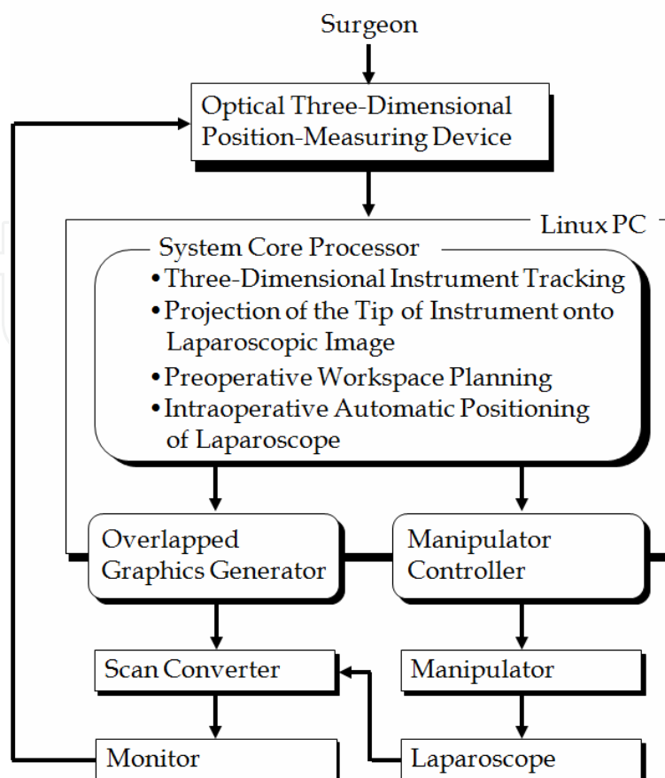
Fig. 12. Control flow of laparoscope robot
