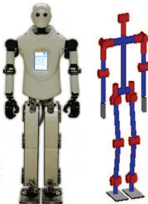
Fig. 4. A humanoid robot AMIO and its degrees of freedom
