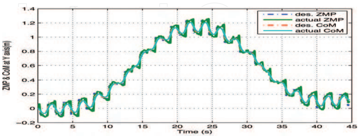
Fig. 16. ZMP and CoM of zig zag walking at Y axis
