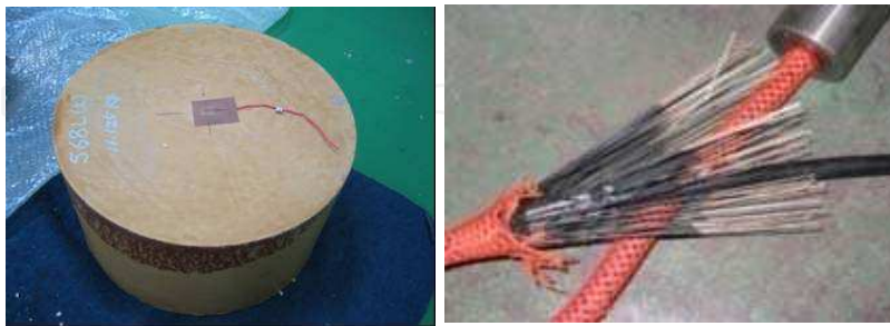
Fig. 1. A prototype of the full ocean depth buoyancy material (left) and the secondary cable made from para-aramid fiber (right).
