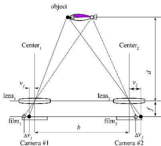
Fig. 5. Camera placement and coordinate system for stereovision.
