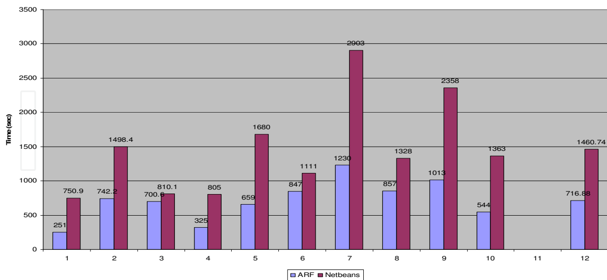
Fig. 11. Scenario creation times: ARF vs. Netbeans
