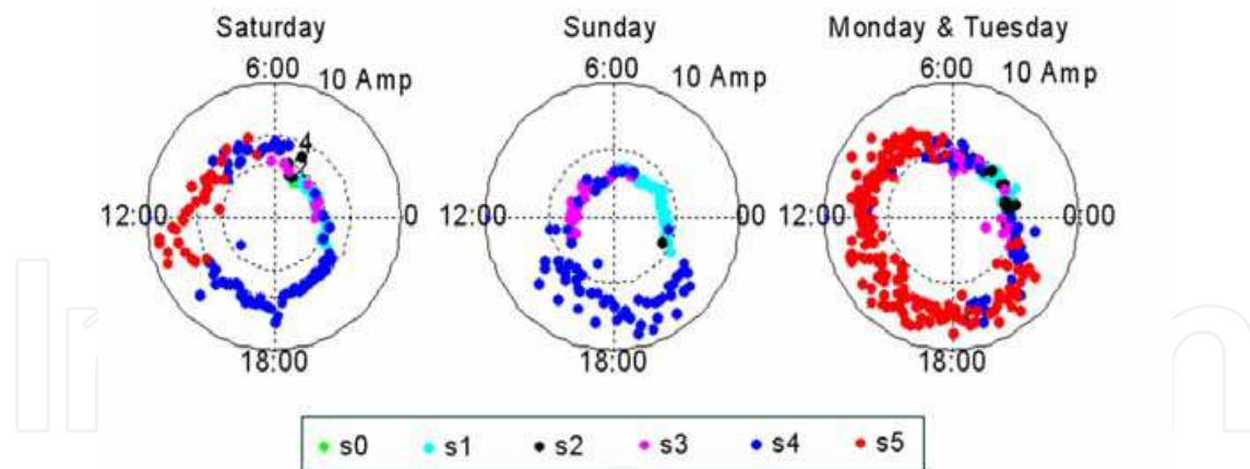
Fig. 14. 5th harmonic current clusters at industrial site for different week days.
