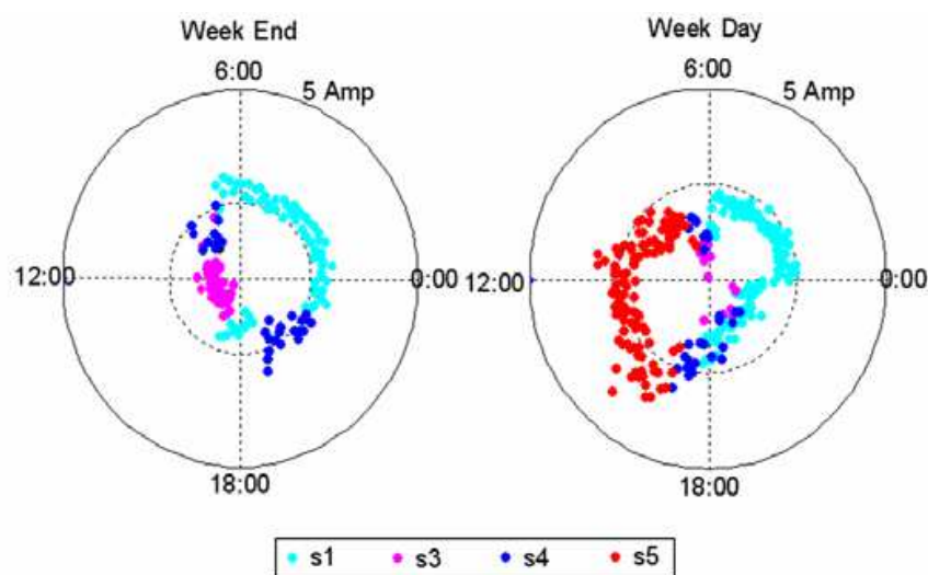
Fig. 15. 5th harmonic current clusters at commercial site for two different week days.
