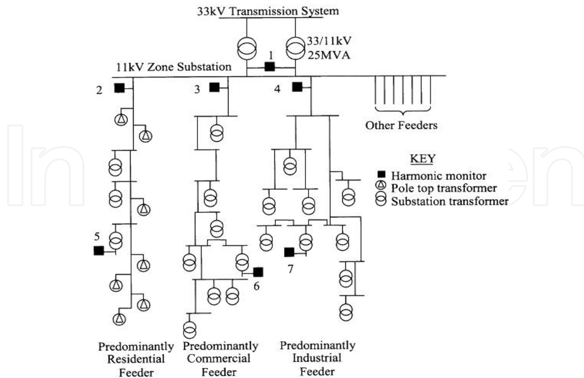
Fig. 1. Single line diagram illustrating the zone distribution system.
