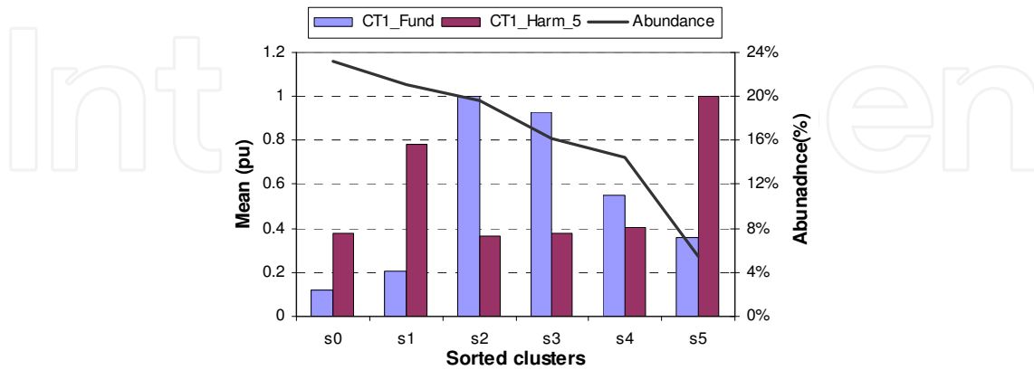
Fig. 5. Fundamentals and 5 th harmonic current clusters in a single phase.
