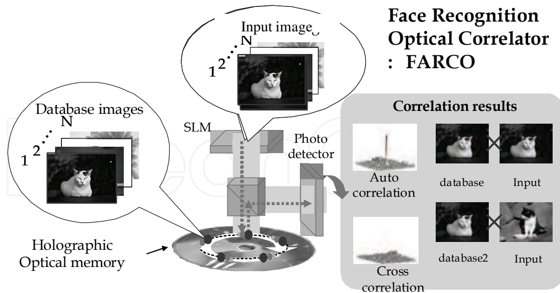
Fig. 8. Optical correlator using holographic optical disc : S-FARCO
