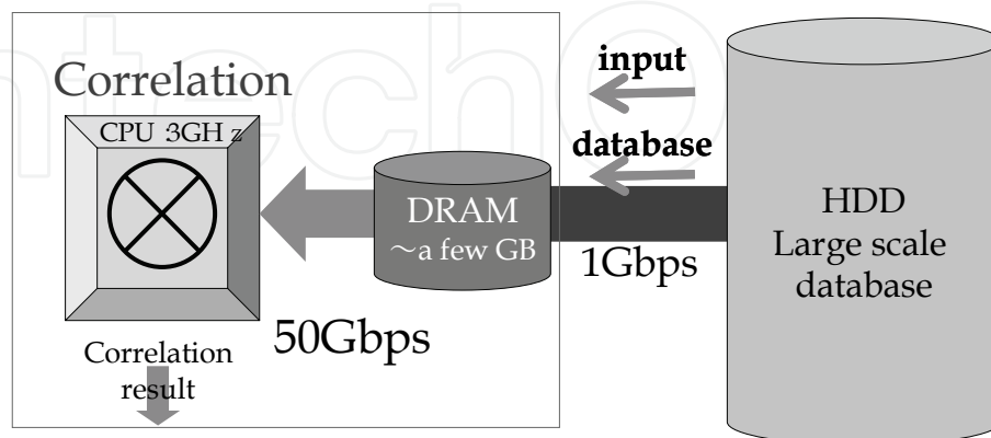
Fig. 6. Conventional search engine
