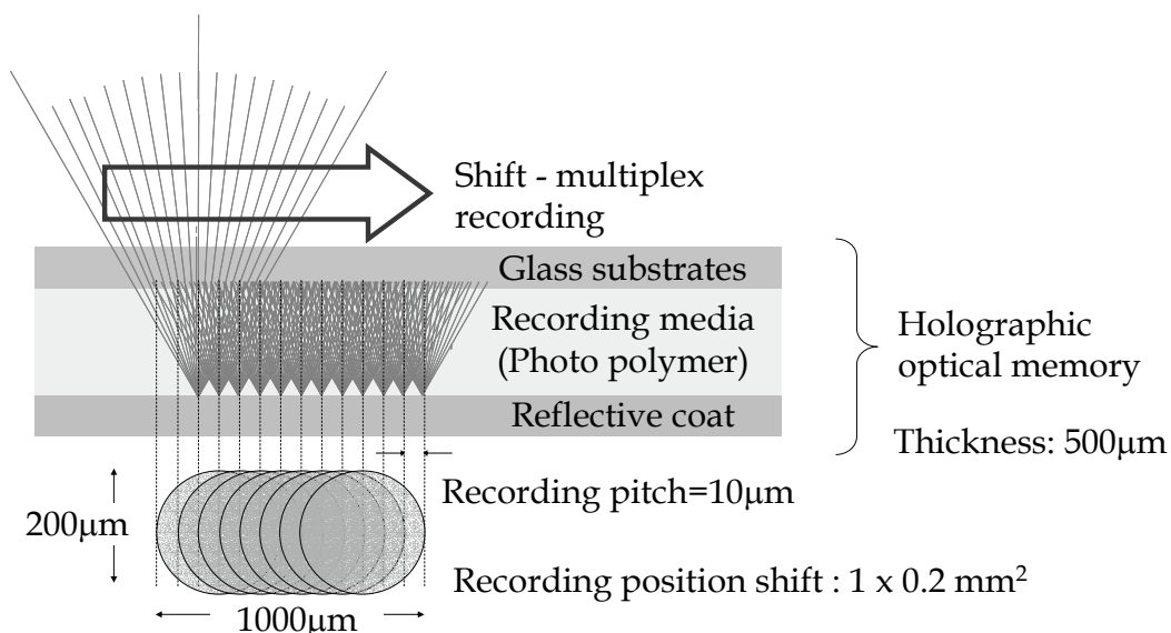
Fig. 12. Multiplex recording method
