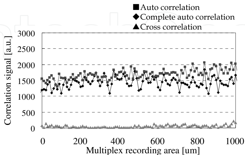
Fig. 13. Experimental results of 100 multiplex memory recording
