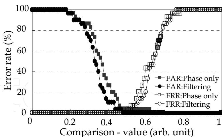
Fig. 5. Results for two kinds of correlation with 64 x 64 pixel
