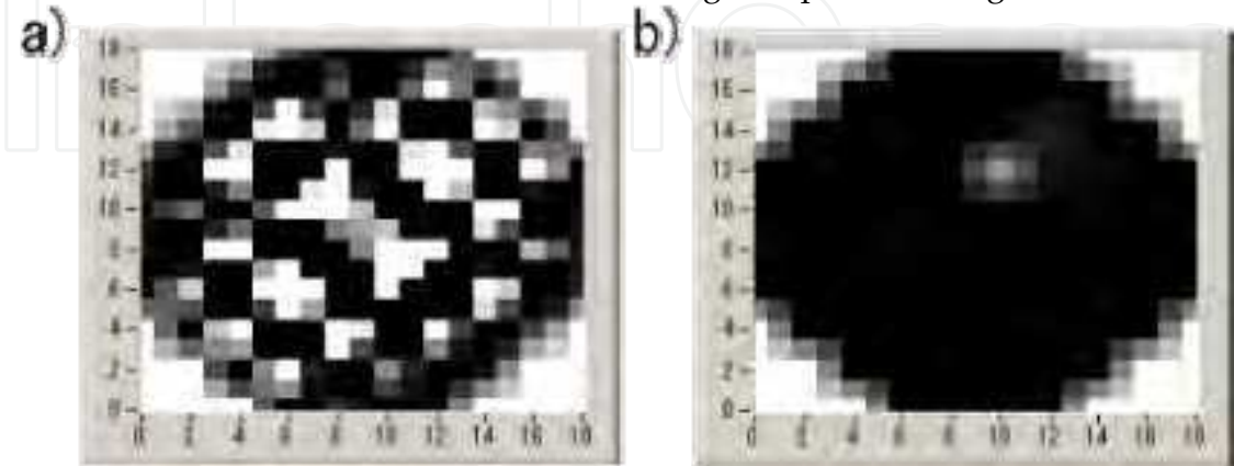
Fig. 7. Comparison between ordinal least square solution and non-negative least square solution from the same input data a) ordinal least square solution, b) non-negative least square solution
