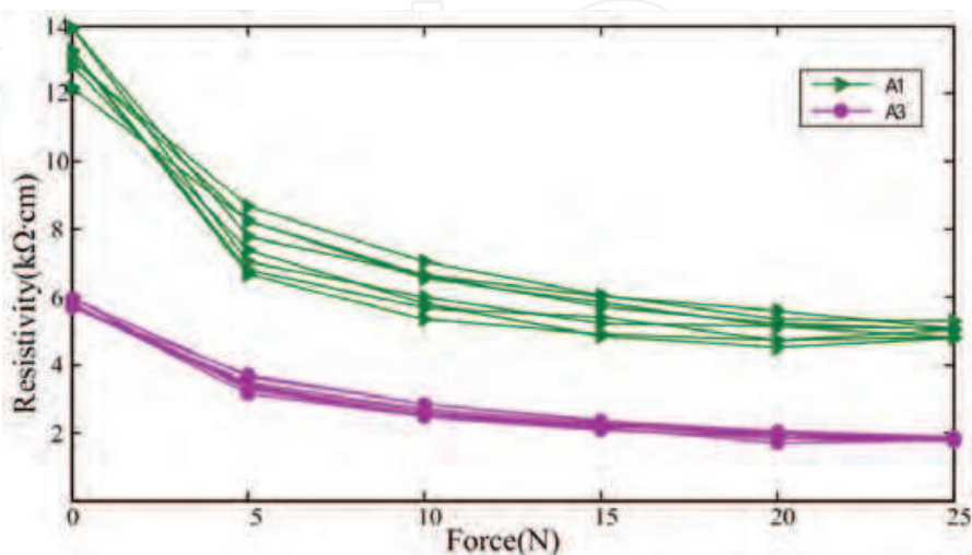
Fig. 8. Reproducibility curves
