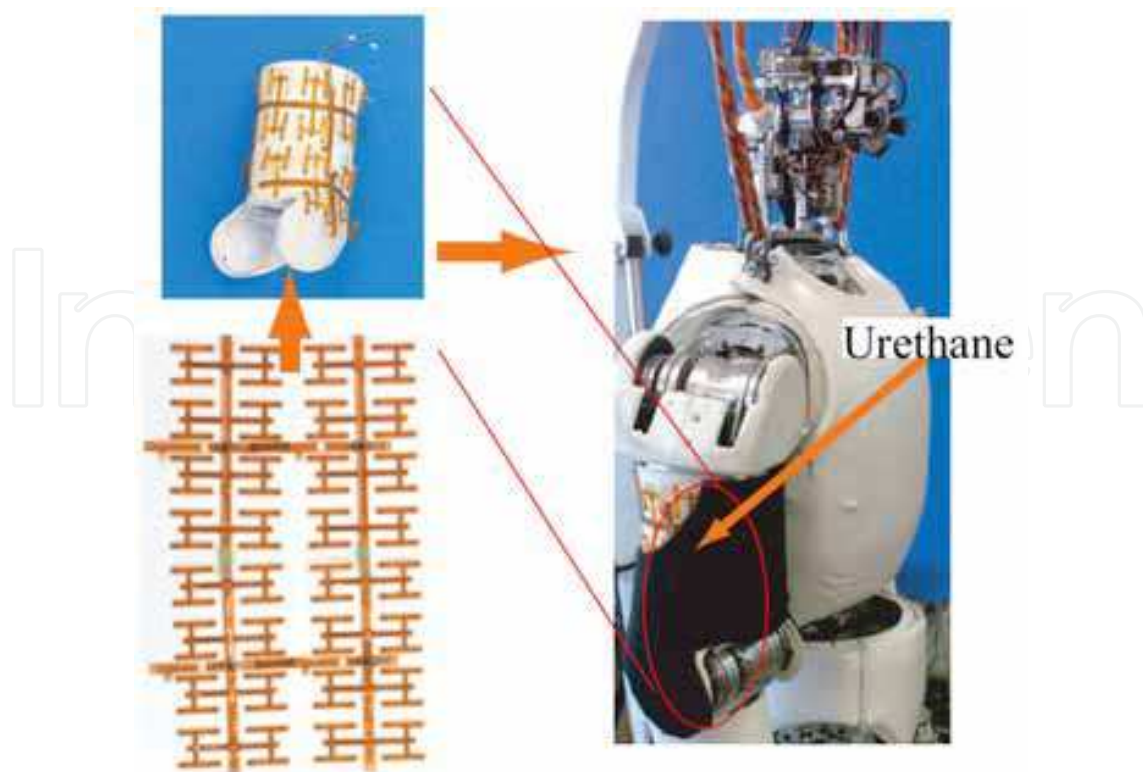
Fig. 9. Integration of the robot skin on the robot (Ohmura 2007).
