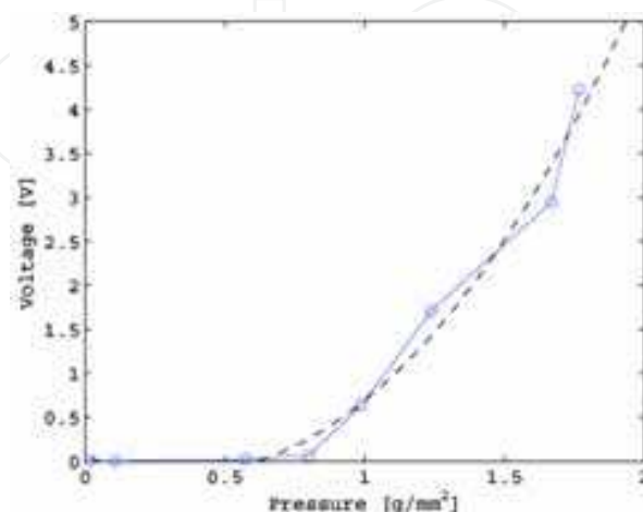
Fig. 23. Pressure to voltage ratio of a generic taxel. Dashed curve is the cubic that approximate the characteristics of the taxel
