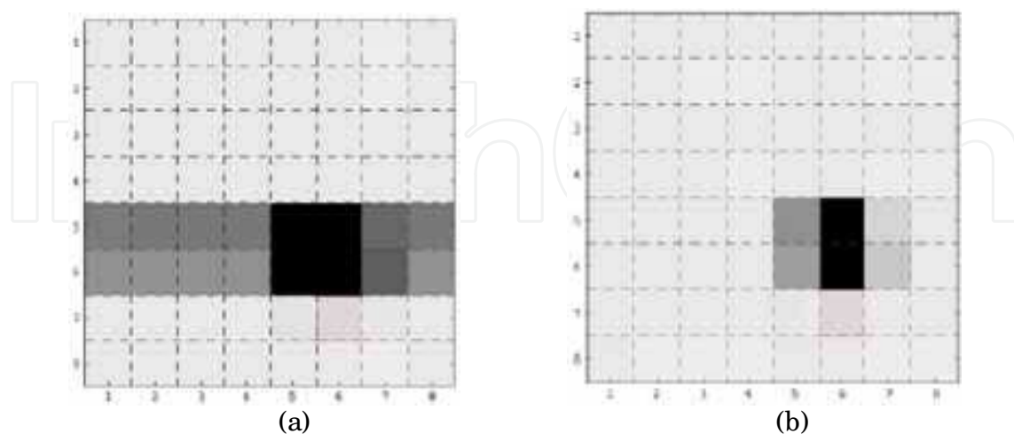
Fig. 21. The tactile image refers to a small cylindrical presser. Fig. a shows the measured pressure distribution using conventional matrix scan. Fig. b shows the tactile image obtained using the proposed compensation method, based on dummy column method , where the false pressure distribution has been removed.
