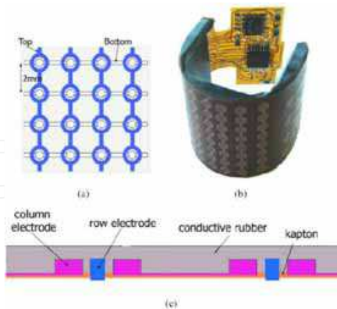
Fig. 19. The electrodes of the tactile sensor are etched on a double layer flex-PCB, and are connected in a matrix configuration (fig. a). The flex circuit conforms to the cylindrical phalange rigid cover (fig. b - resistive rubber not shown here). Fig. c: section view of the tactile sensor. Row electrodes are encircled by column electrodes.
