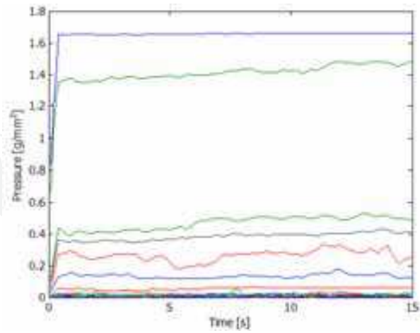
Fig. 25. Time behaviour of the taxels.
