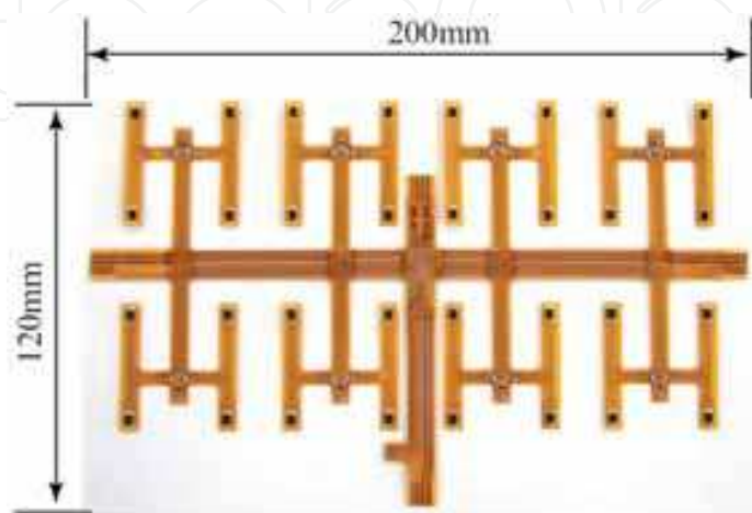
Fig. 8. Tactile sensor sheet (Ohmura 2007)
