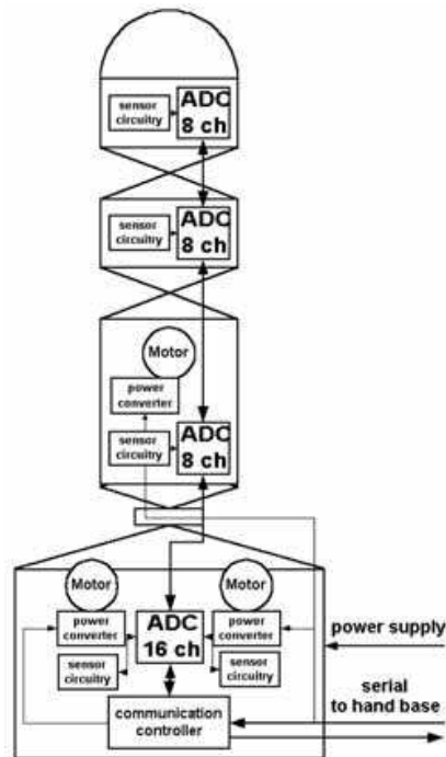
Fig. 2. Embedded electronics of the DLR-II finger (Butterfass et al. 2001).
