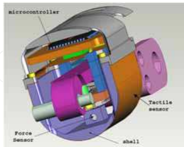
Fig. 17. CAD model of the whole phalange, with the force sensor, the tactile transducer and MCU board.
