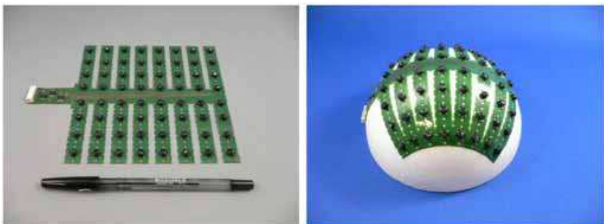
Fig. 10. Tactile sensors for the RI-MAN humanoid robot (Mukai, 2008).
