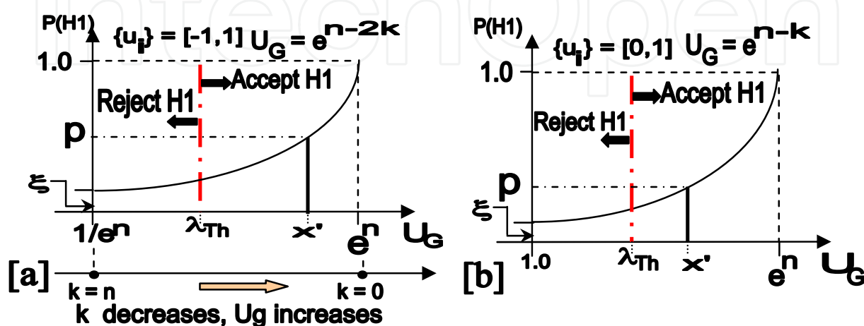
Fig. 2. HEBTEM with multiplicative model of data fusion for [a] \{u_i\}=[-1,1] & [b] u_i=[0,1]
