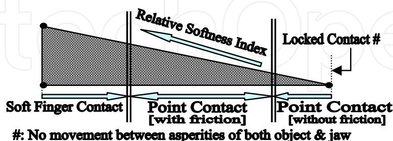
Fig. 15. Schematic view of the distribution of contact zones as contrasted with RSI
