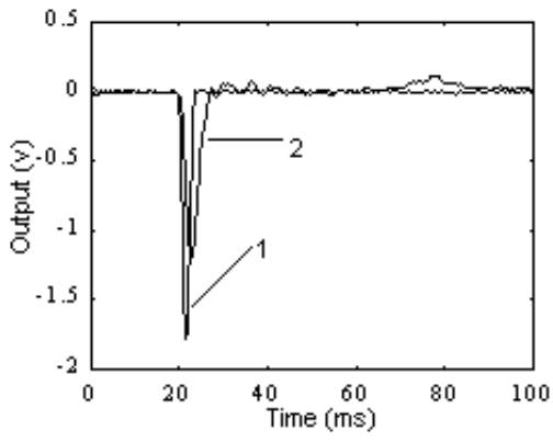
Fig. 6-18 Compensation result of NLC using linear approach compared with the input signal (1) impulse input, (2) compensation result
