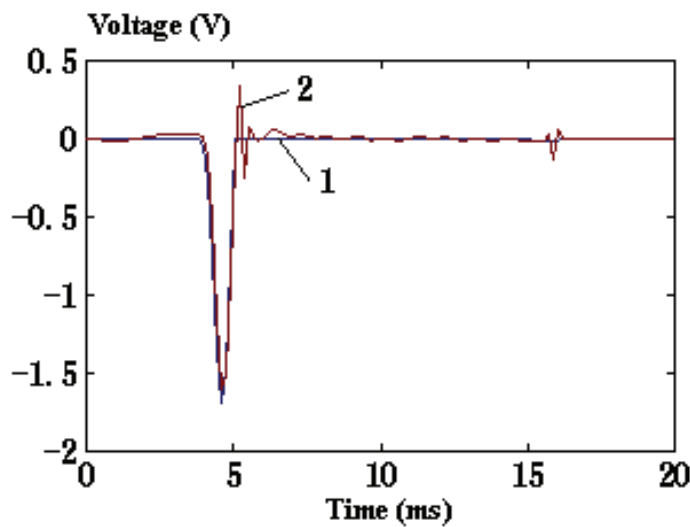
Fig. 5-3 (a) Decoupling and compensating result of direction Z
