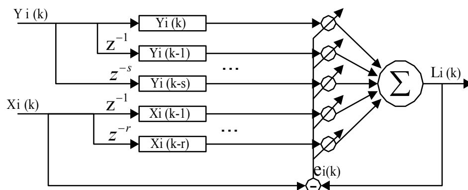
Fig. 5-2 Schematic of modeling by FLANN
