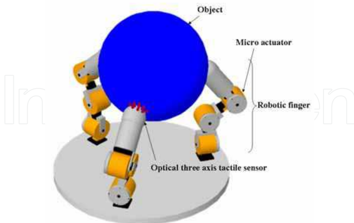
Fig. 2. Rendering of a three fingered hand equipped with optical three-axis tactile sensors
