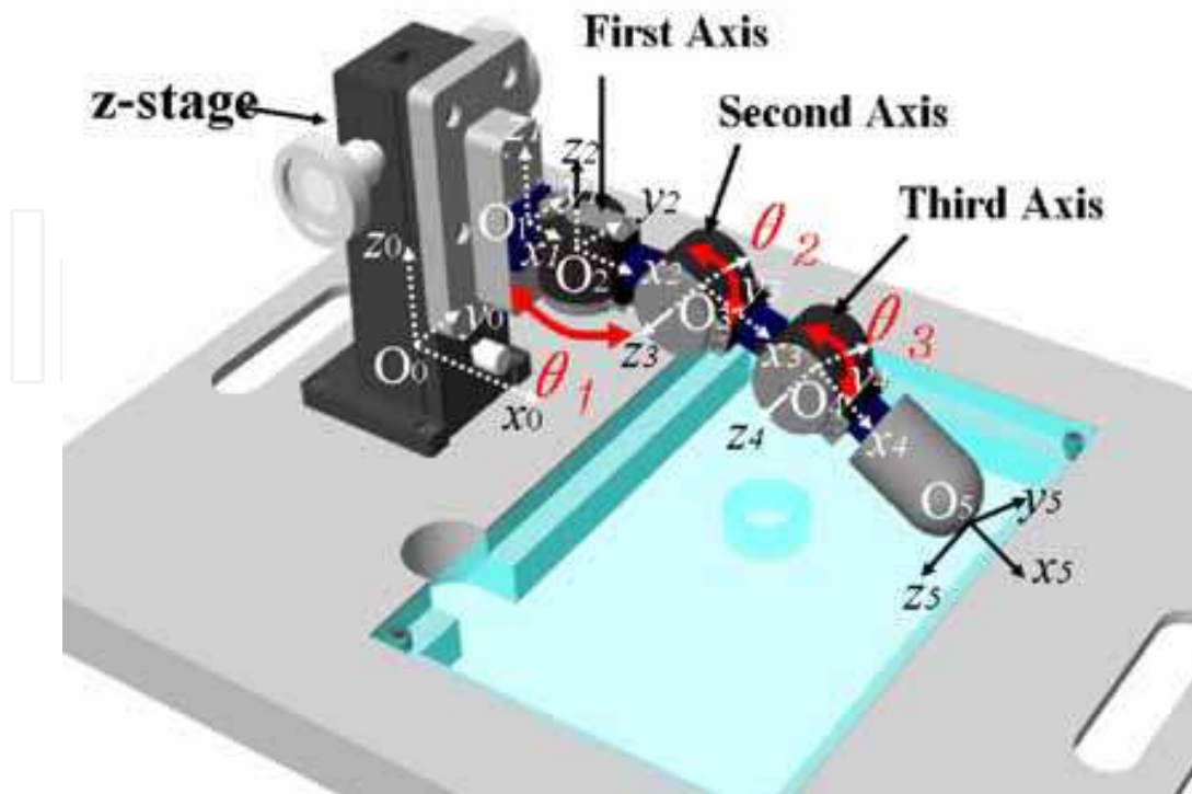
Fig. 16. Robotic finger equipped with a three-axis tactile sensor
