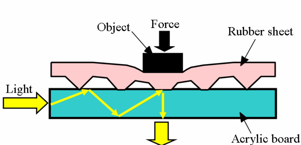
Fig. 1. Conventional optical tactile sensor
