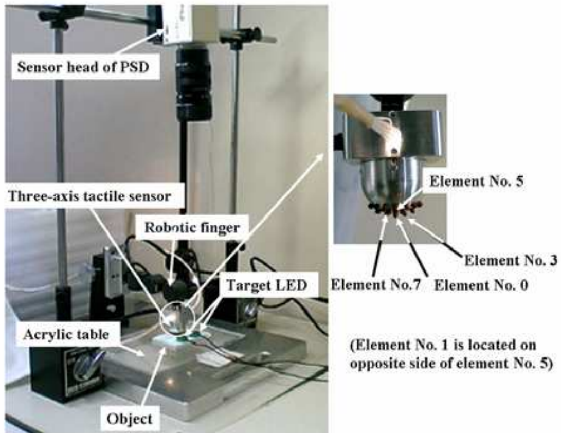
Fig. 19. Set up for object manipulations
