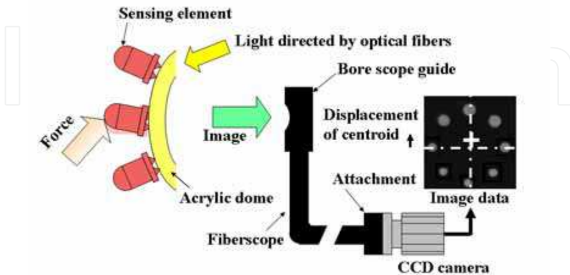
Fig. 4. Principle of three-axis tactile sensor system
