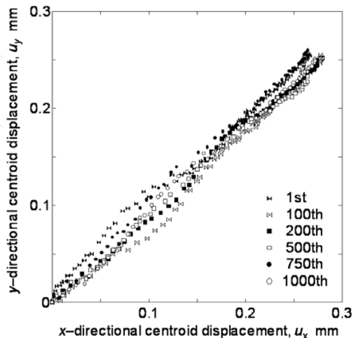
Fig. 14. Repeatability of shearing force detection
