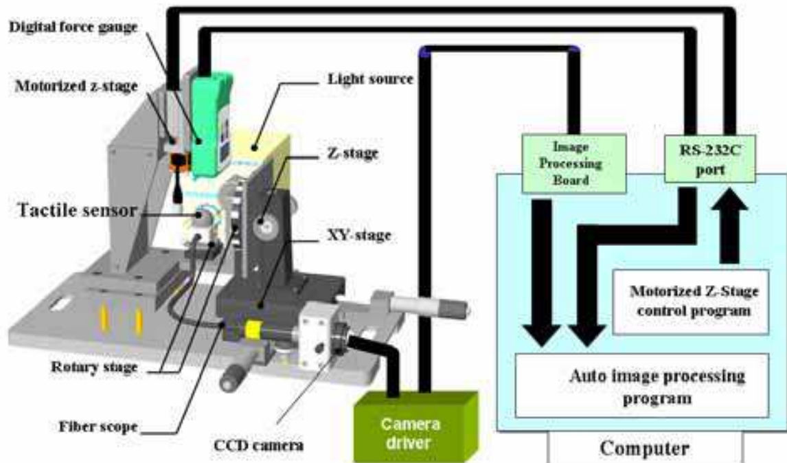
Fig. 6. Loading machine and tactile data processing system
