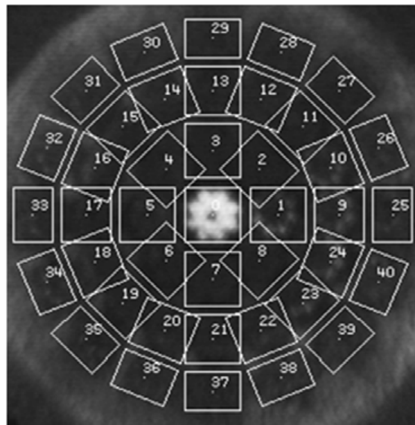
Fig. 7. Address of sensing elements
