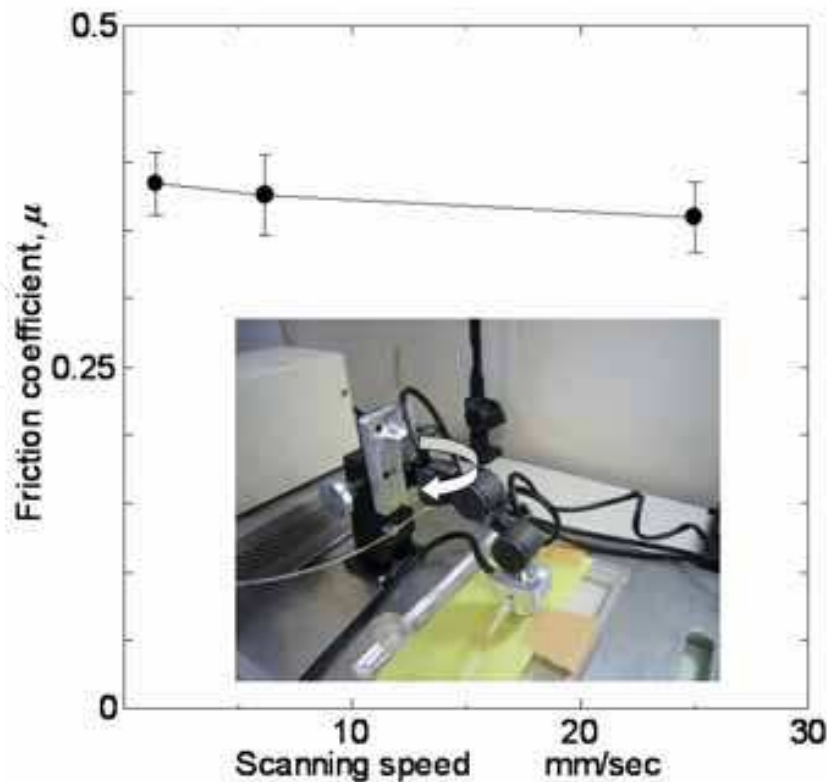
Fig. 18. Dependence of friction coefficient on scanning velocity
