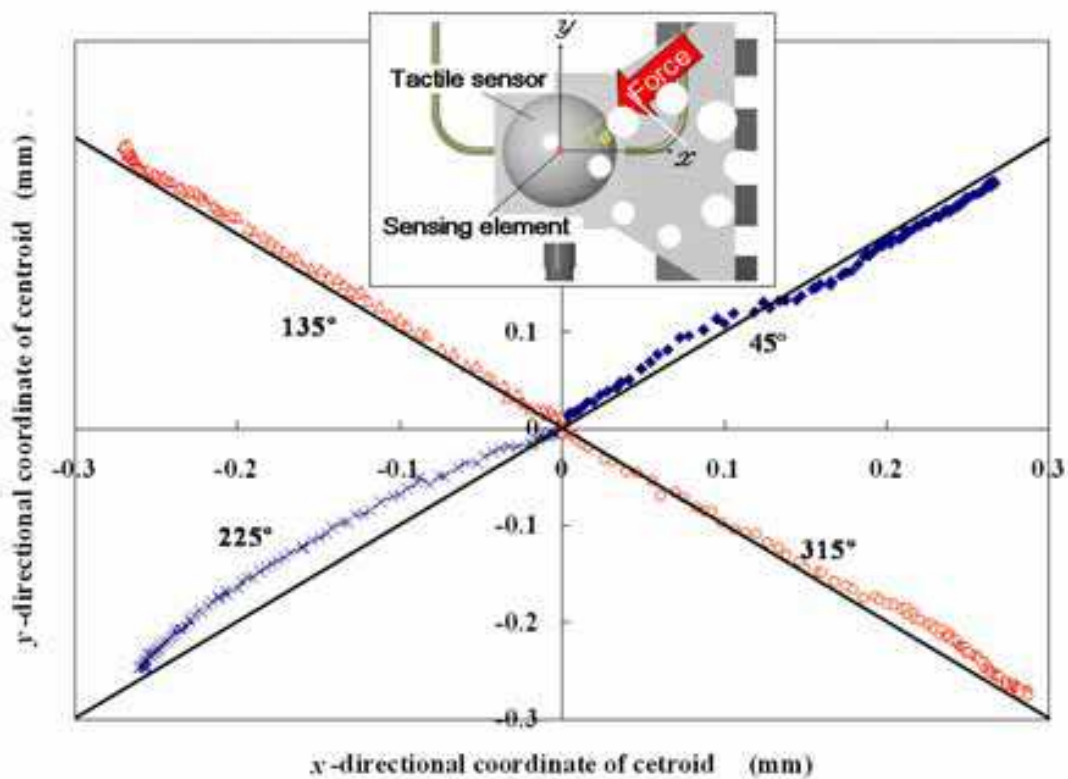
Fig. 12. Precision of two-dimensional shearing force detection
