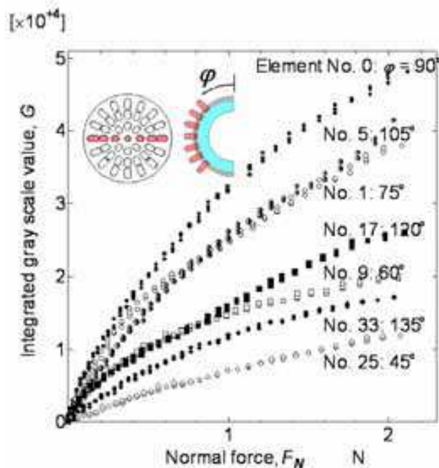
Fig. 8. Relationship between applied force and grayscale value
