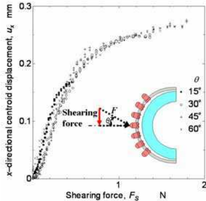
Fig. 11. Relationship between centroid displacement and applied shearing force
