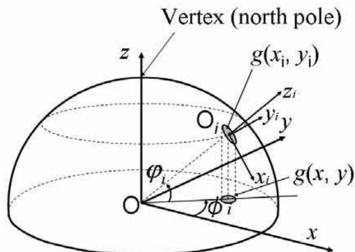
Fig. 5. Relationship between spherical and Cartesian coordinates
