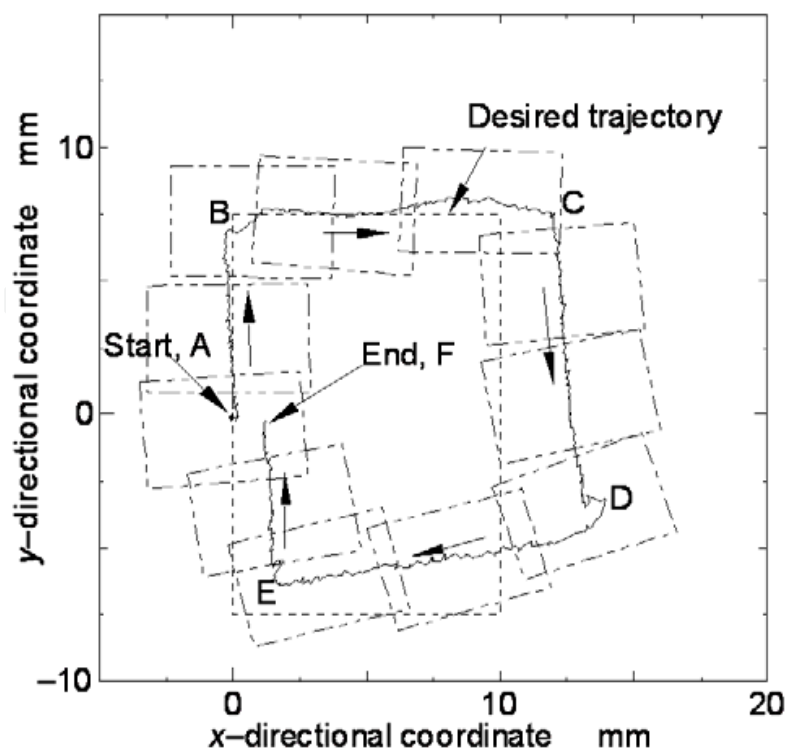
Fig. 20. Manipulation of parallelepiped object
