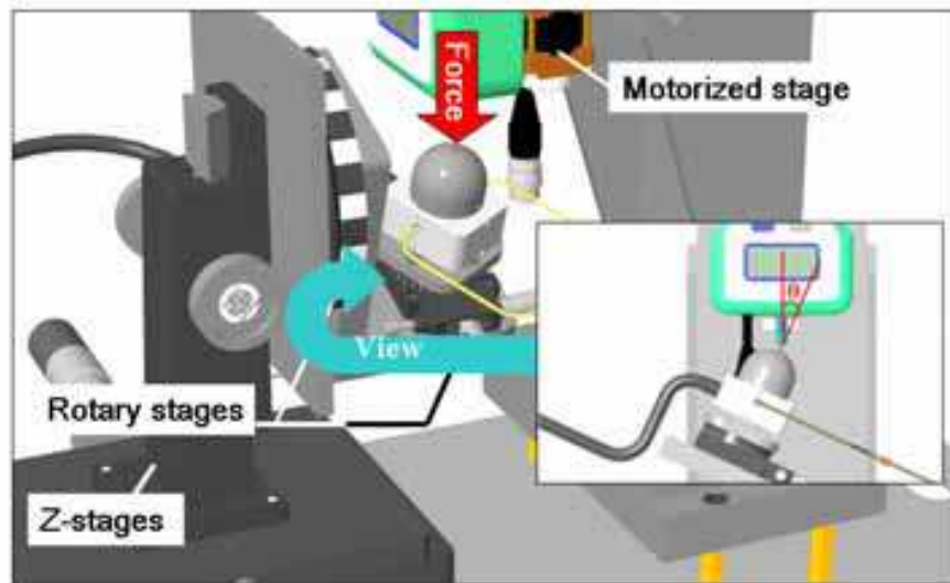
Fig. 9. Generation of shearing force component
