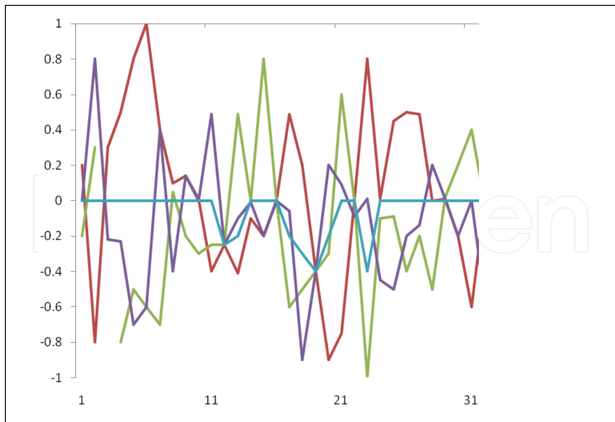
Fig. 7. Competitive agent parameter optimisation. Averaged over 30 hands
