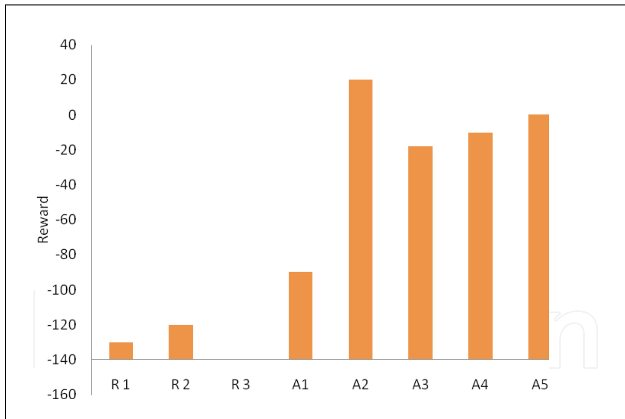
Fig. 8. Competitive agent parameter optimisation. Averaged over 30 hands
