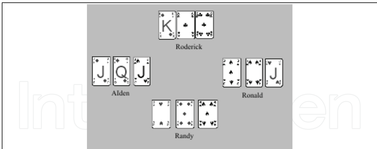
Fig. 11. Agent bluffing
