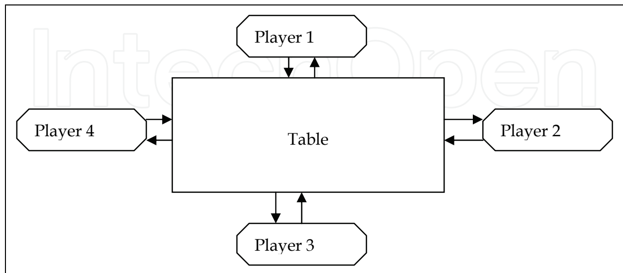
Fig. 1. System interactions
