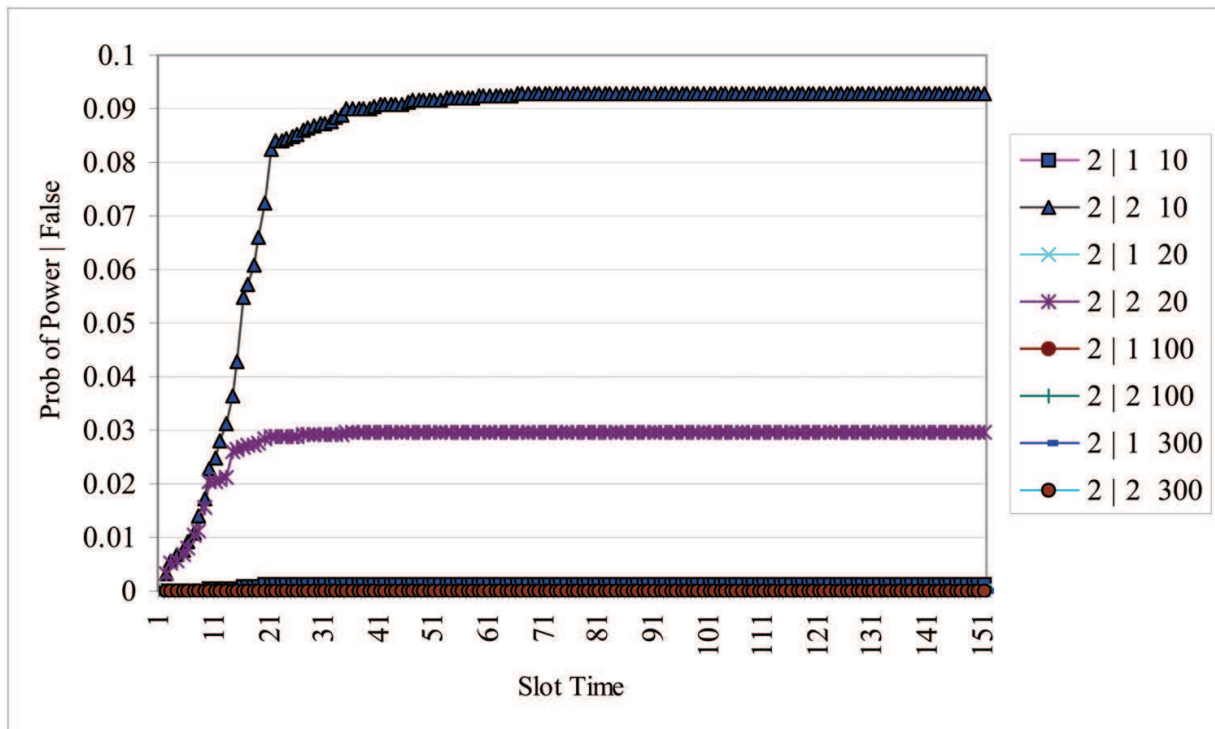
Fig. 2. Power & False Alarm Curves for 0.1 \rightarrow 0.25 Monitoring Algorithm at the Fusion Center, for 30 Sensors. Legend: 2 | 1 : False Alarm 2 | 2 : Power
