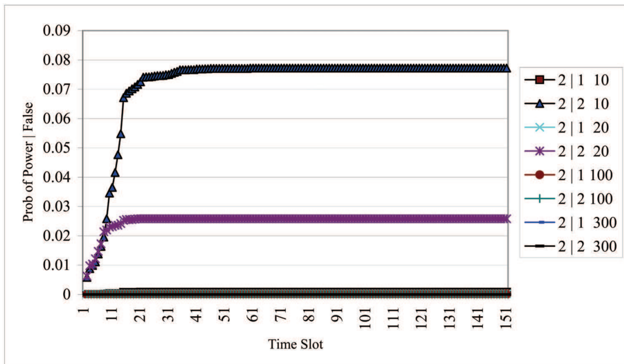
Fig. 3. Power & False Alarm Curves for 0.1 \rightarrow 0.25 Monitoring Algorithm at the Fusion Center, for 50 Sensors. Legend : 2 | 1 : False Alarm 2 | 2 : Power
