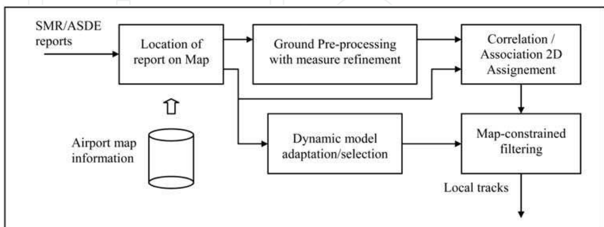
Fig. 17. SMR/ASDE pre-processing synoptic
