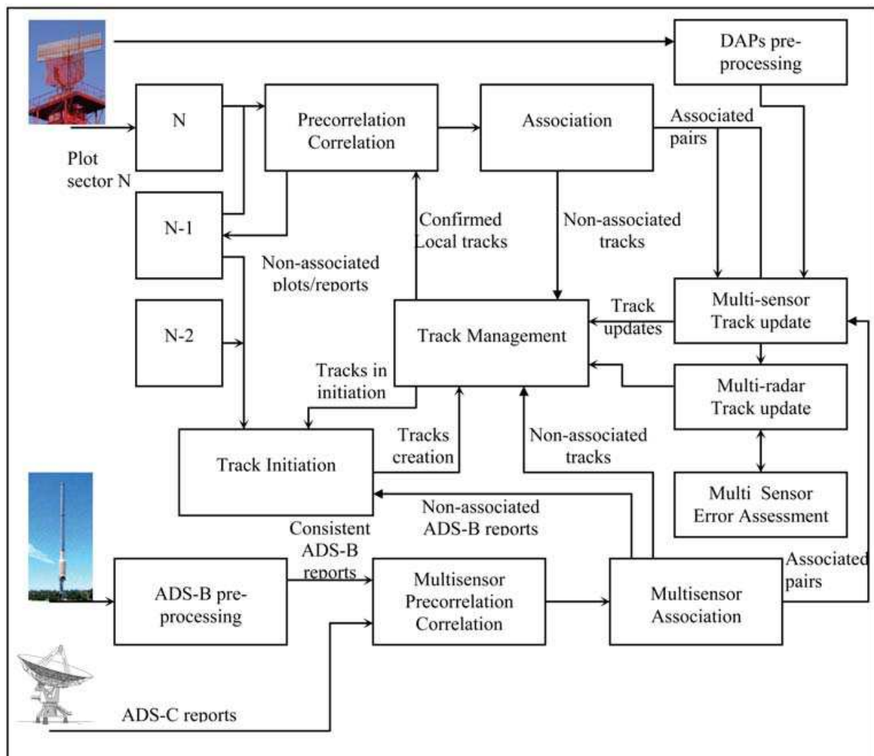
Fig. 14. Radar / ADS-B / ADS-C data fusion architecture
